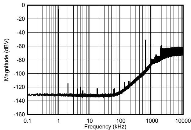
Figure 7-1. Quantization Noise Shaping
