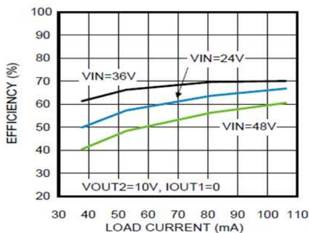
Figure 21. Efficiency at 750 kHz, V_{OUT1} = 10 V
