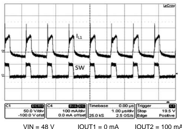
Figure 22. Steady-State Waveform
