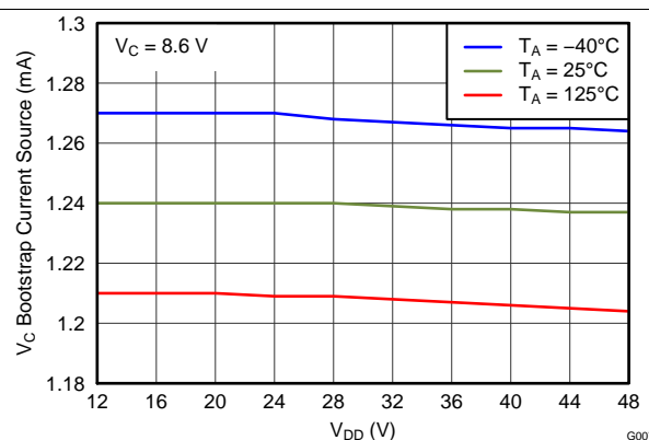
Figure 11. VC Bootstrap Current Source vs Supply Voltage
