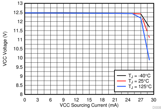
Figure 7-8. Converter Startup Voltage vs Current
