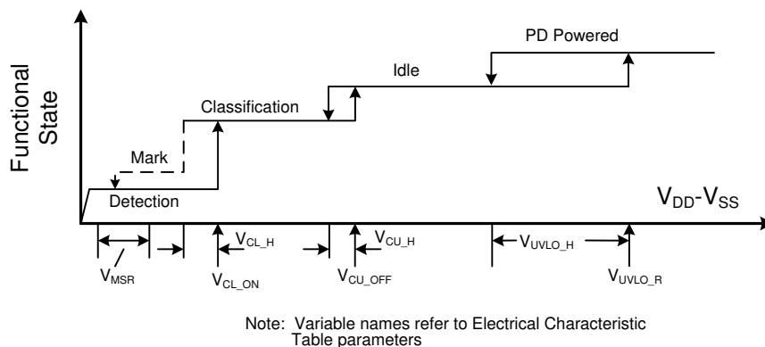
Figure 8-6. Threshold Voltages
