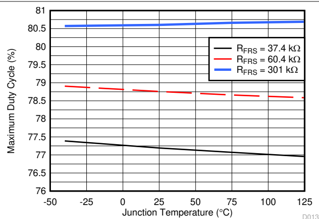
Figure 7-13. Maximum Duty Cycle vs Temperature
