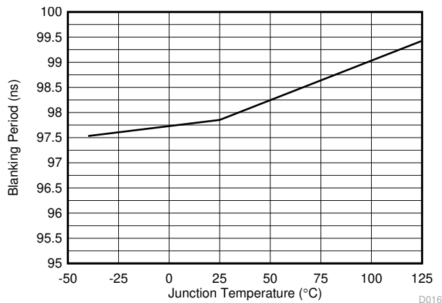
Figure 7-16. Blanking Period vs Temperature
