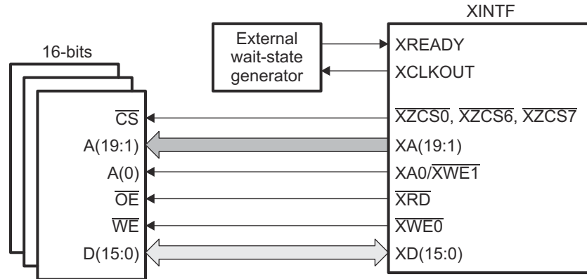
图 8-21. Typical 16-Bit Data Bus XINTF Connections
