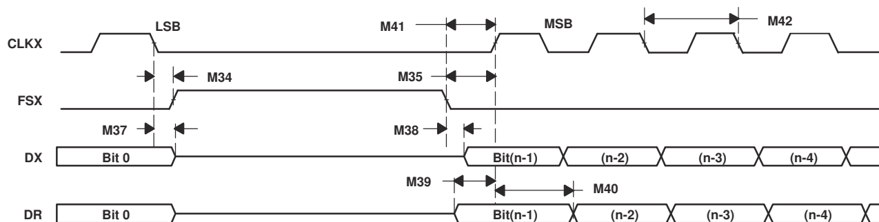
图 7-24. McBSP Timing as SPI Master or Slave: CLKSTP = 11b, CLKXP = 0
