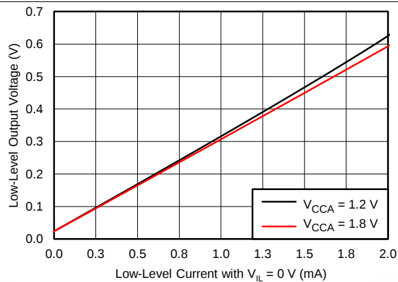
Figure 1. Low-Level Output Voltage (VOL(DATxB)) vs Low-Level Current (IOL(DATxA))
