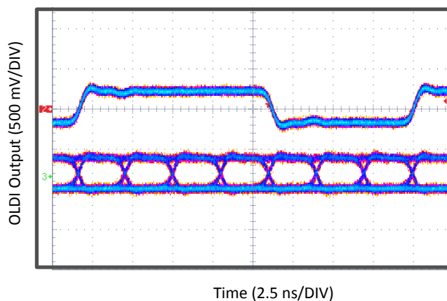
Figure 6-16. OpenLDI Output With 96-MHz Clock
