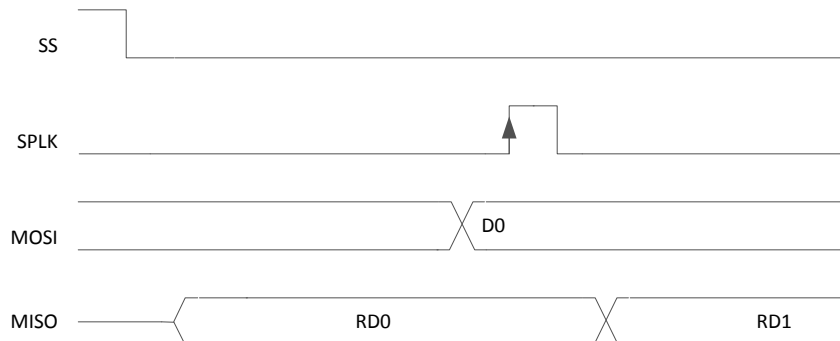
Figure 7-5. Reverse Channel SPI Read
