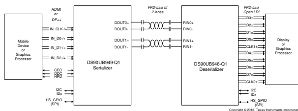
Figure 3-1. Typical Application
