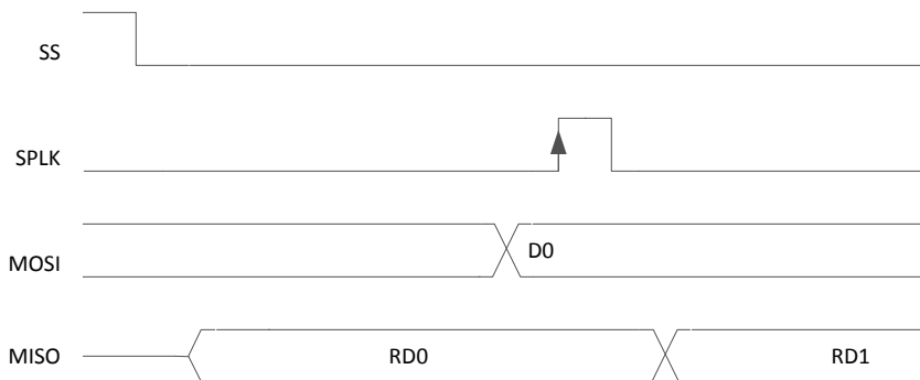
Figure 7-3. Forward Channel SPI Read
