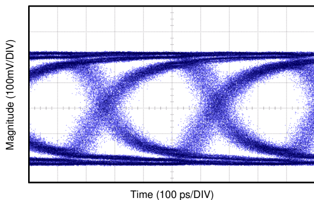
Figure 6-15. Deserializer Eye Diagram With 2.6-Gbps FPD-Link III Rate
