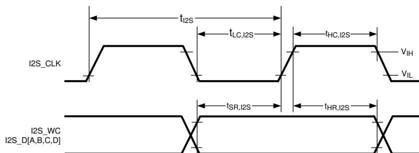
Figure 6-14. I2S Timing
