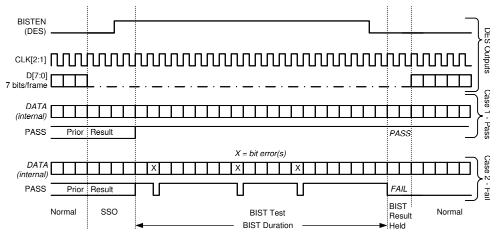
Figure 7-14. BIST Waveforms
