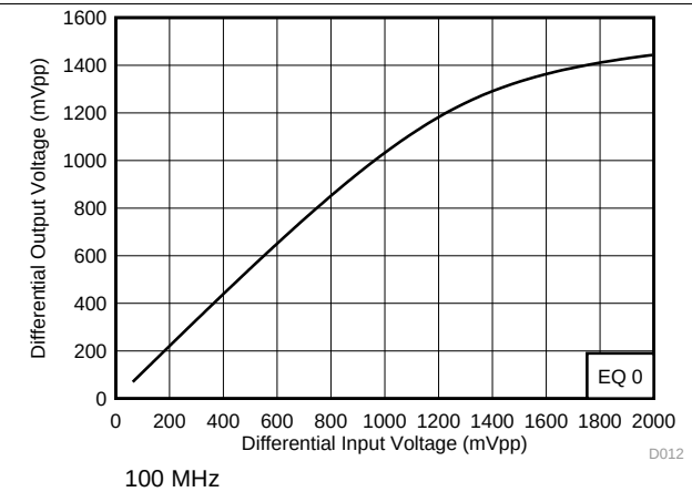
图 18. Upstream-to-Downstream Linearity Performance at 100 MHz
