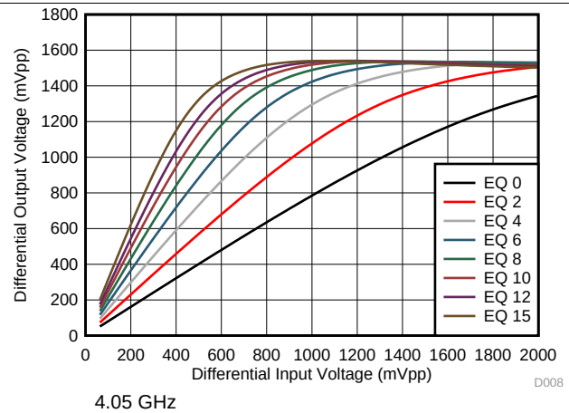
图 14. Downstream-to-Upstream Linearity Performance at 4.05 GHz
