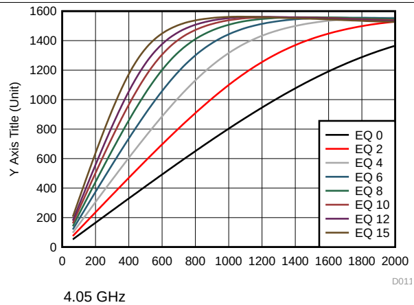
图 17. Upstream-to-Downstream Linearity Performance at 4.05 GHz
