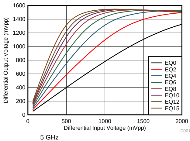
图 13. Downstream-to-Upstream Linearity Performance at 5 GHz
