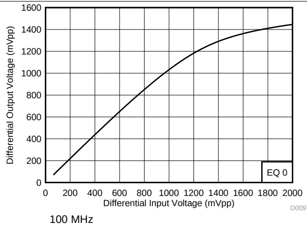
图 15. Downstream-to-Upstream Linearity Performance at 100 MHz
