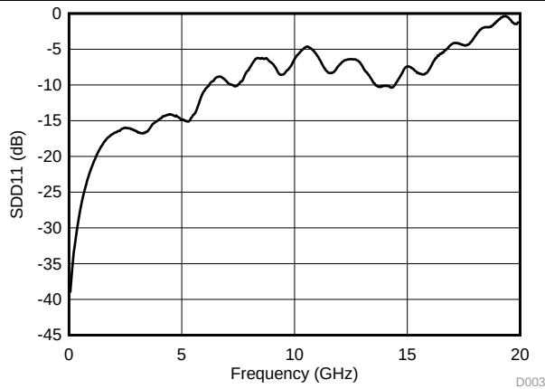
图 9. Input Return Loss Performance of the Downstream Ports
