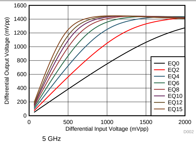
图 16. Upstream-to-Downstream Linearity Performance at 5 GHz
