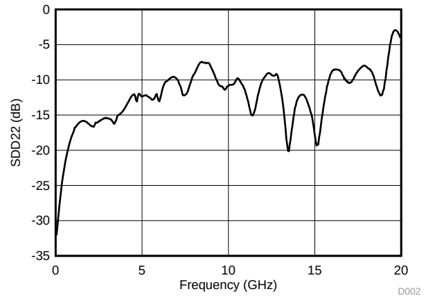
图 10. Output Return Loss Performance of the Downstream Ports
