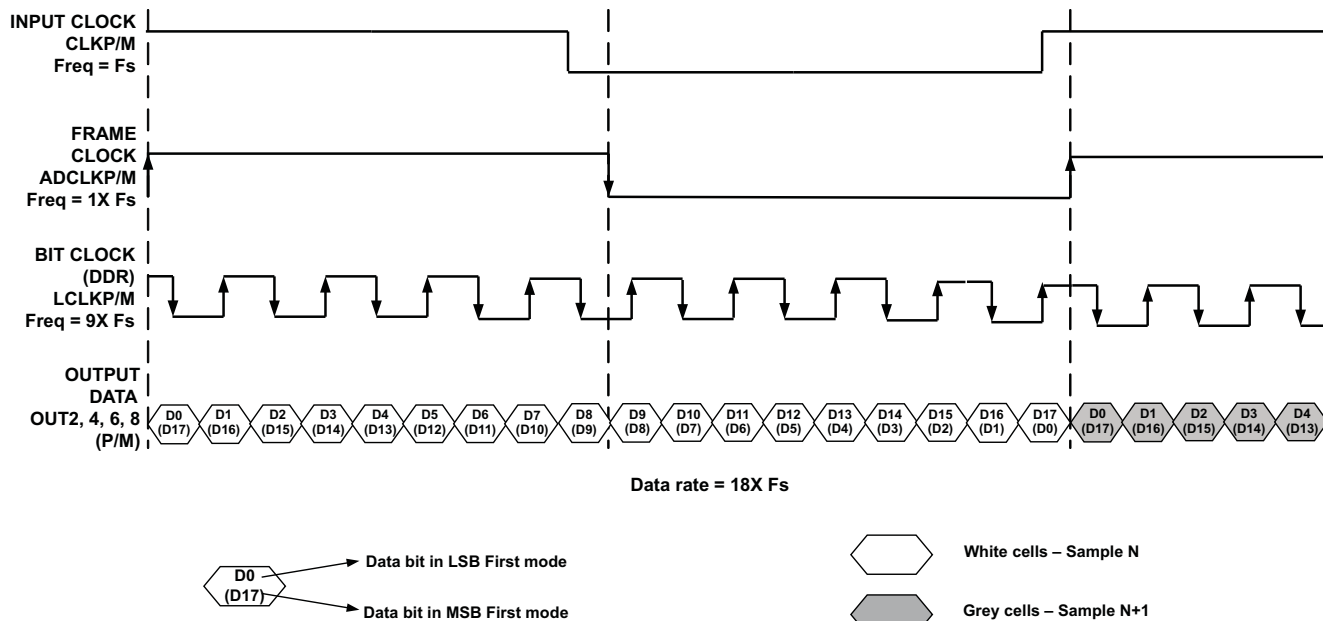
Figure 56. LVDS Output Interface, 1-Wire, 18× Serialization
