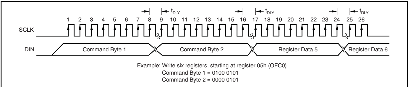
Figure 55. Write Register Data (Table 22 shows t_{DLY} )
