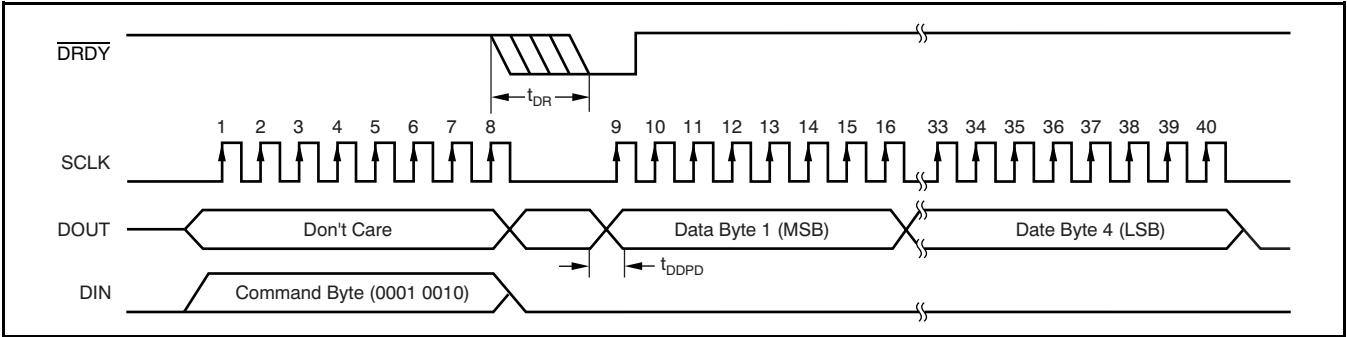
Figure 48. Read Data By Command, RDATA ( t_{DDPD} timing is given in Table 15)
