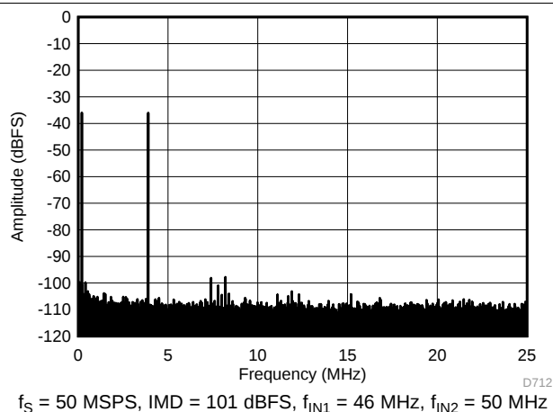
Figure 111. FFT for Two-Tone Input Signal ( -36\text{ dBFS} at 46\text{ MHz} and 50\text{ MHz} )
