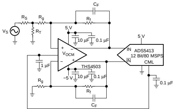
Figure 32. Using the THS4503 With the ADS5413
