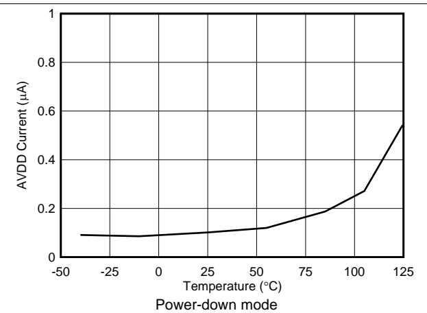
图 21. Analog Supply Current vs Temperature
