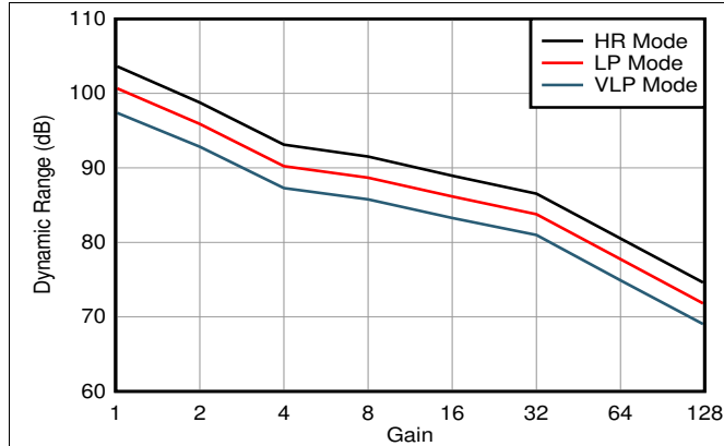
图 10. Dynamic Range vs Gain Across Power Modes
