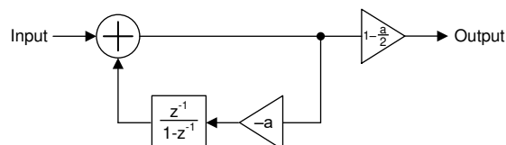
图 32. DC Block Filter Topology
