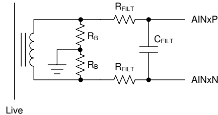
图 95. Current Measurement Front-End
