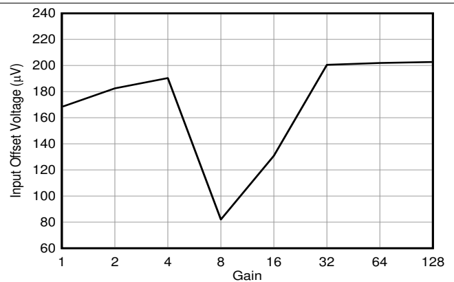
图 5. Input Offset Voltage vs Gain
