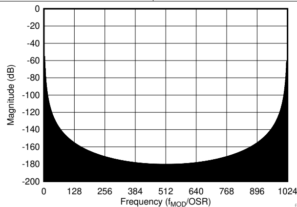
图 28. Sinc 3 Digital Filter Response, OSR 1024, Stop-Band Detail
