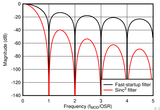
图 29. Fast-Settling and Sinc³ Digital Filter Response
