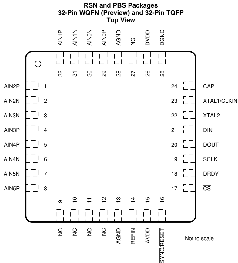
Pin Functions
