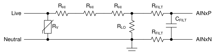
图 94. Voltage Measurement Front-End
