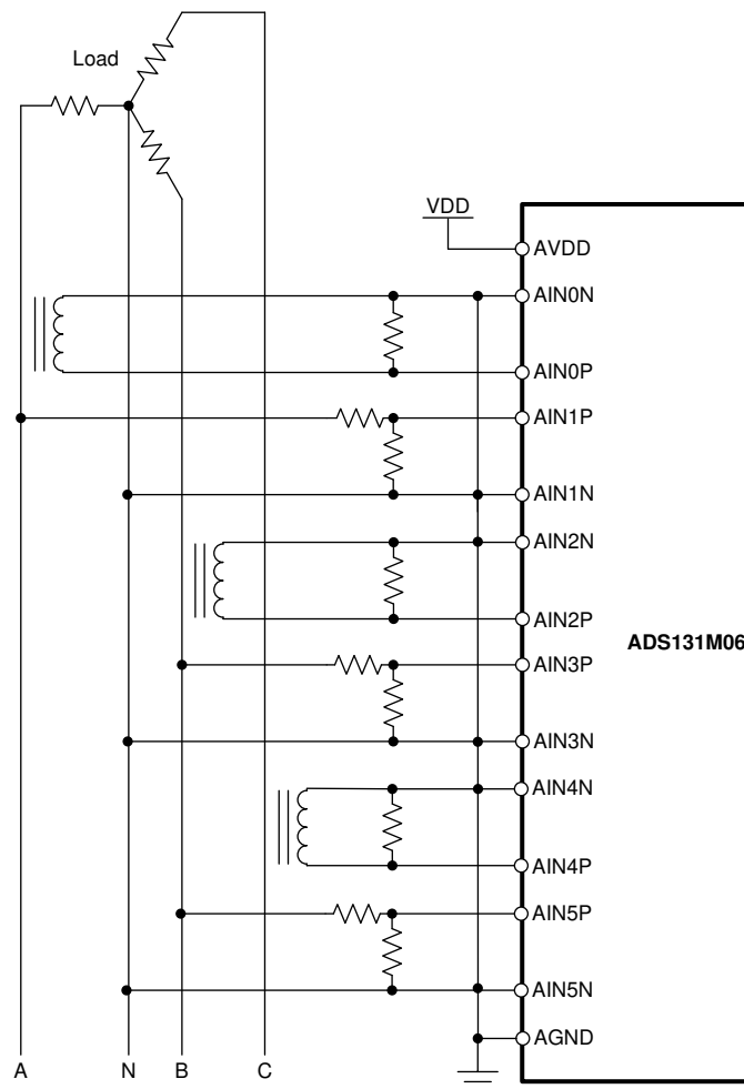
图 91. Three-Phase Current and Voltage Measurement Front-End
