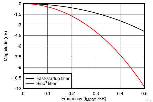
图 30. Fast-Settling and Sinc³ Digital Filter Response, Pass-Band Detail
