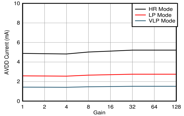
图 17. AVDD Current vs Gain
