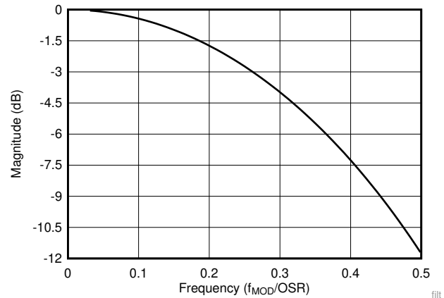
图 27. Sinc 3 Digital Filter Response, Pass-Band Detail
