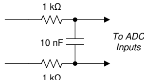
图 89. Recommended Antialiasing Circuitry
