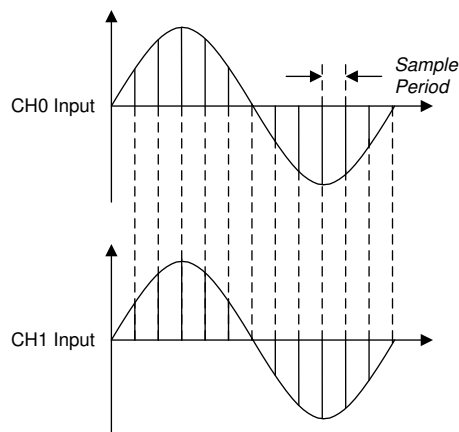
图 33. Two Channel Outputs With Equal Phase Settings
