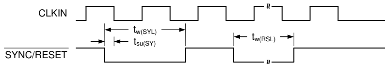
图 2. SYNC/RESET Timing Requirements
