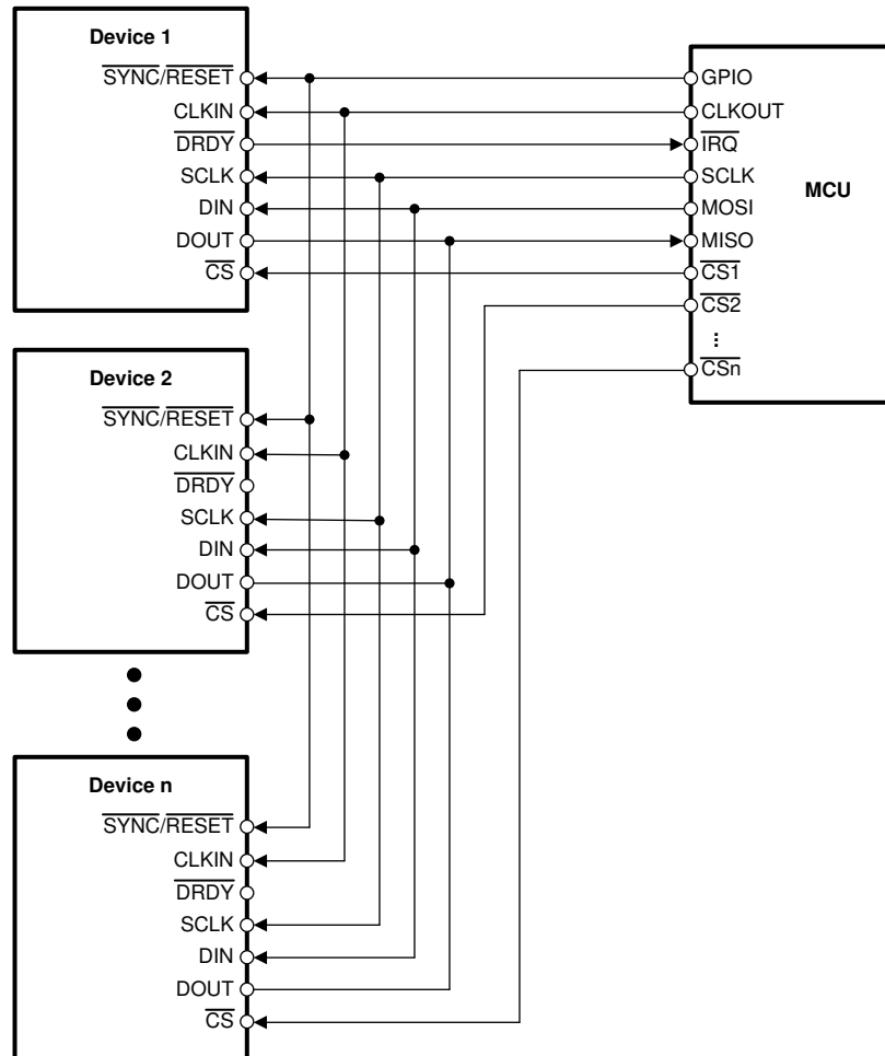
图 92. Multiple Device Configuration
