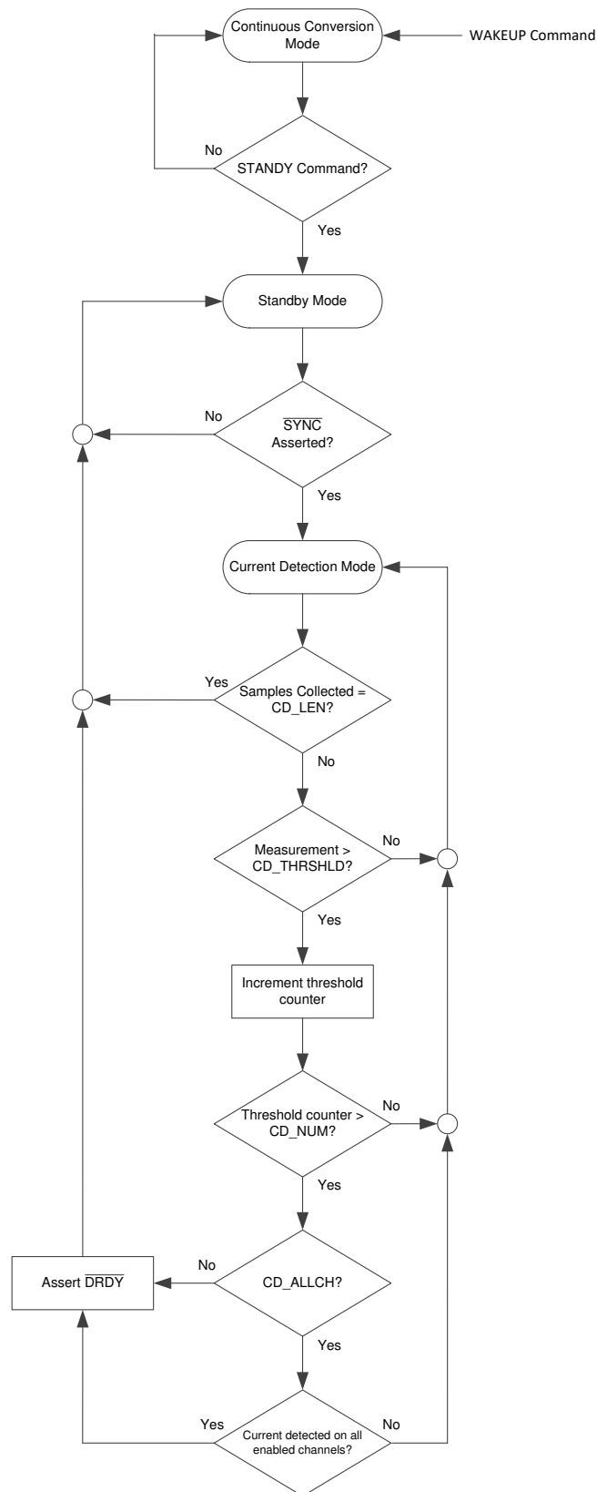
图 39. Current-Detect Mode Flow Chart
