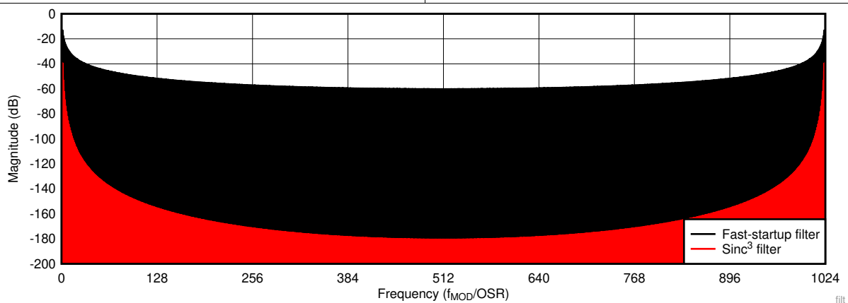
图 31. Fast-Settling and Sinc³ Digital Filter Response, OSR 1024, Stop-Band Detail
