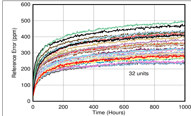
图 22. Long-Term Reference Drift
