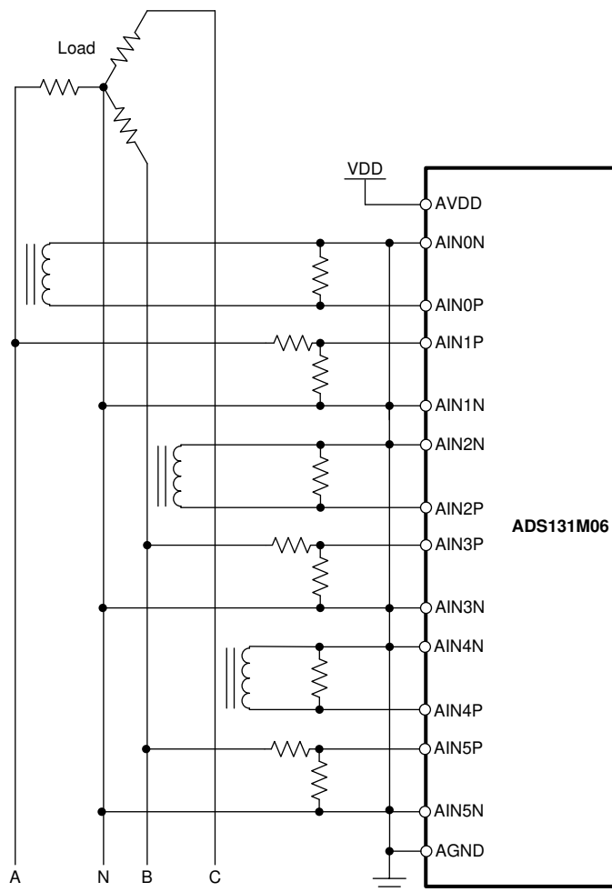
图 93. Three-Phase Metrology Design Front-End
