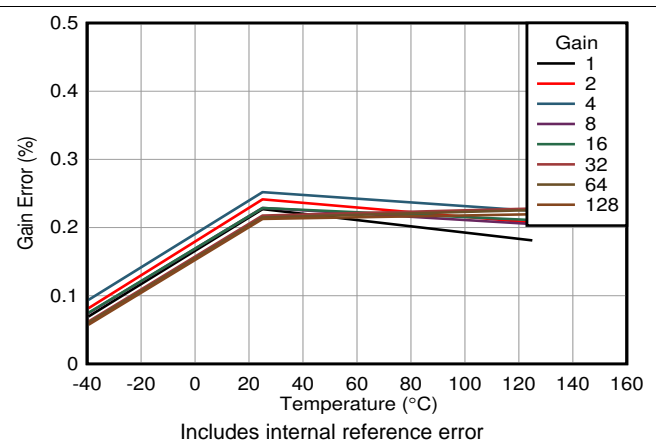
图 7. Gain Error vs Temperature
