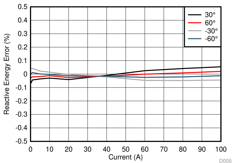
图 97. Cumulative Reactive Energy % Error Versus Current
