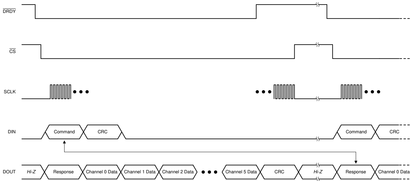
图 40. Typical Communication Frame
