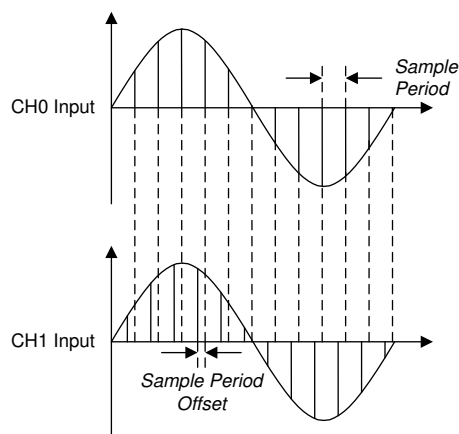
图 34. Channel 1 With a Positive Sample Phase Shift With Respect to Channel 0
