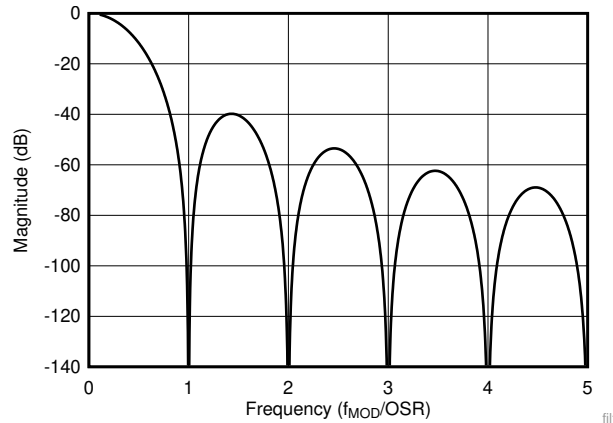
图 26. Sinc 3 Digital Filter Response
