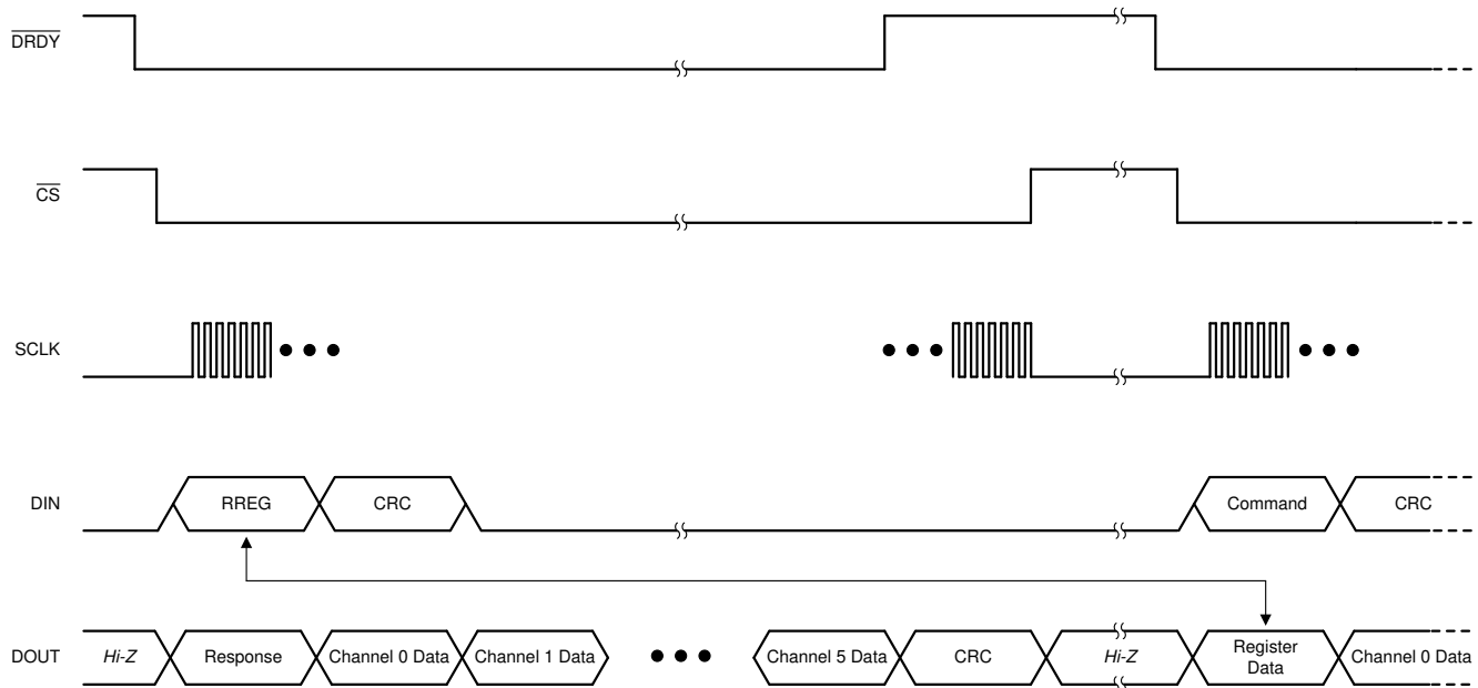
图 45. Reading a Single Register
