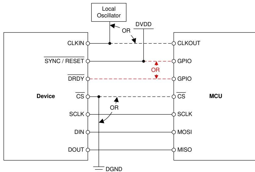
图 90. Minimum Connections Required to Operate the ADS131M06
