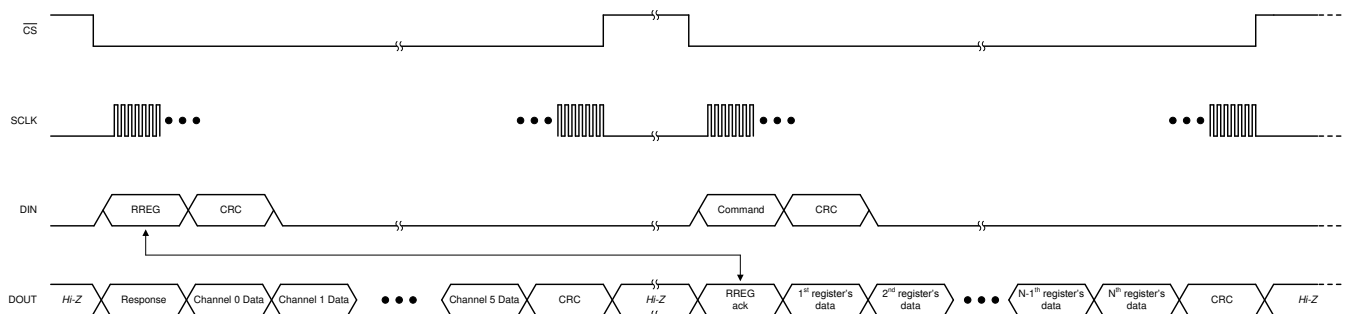
图 46. Reading Multiple Registers
