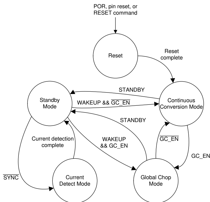
图 38. State Diagram Depicting Device Functional Modes
