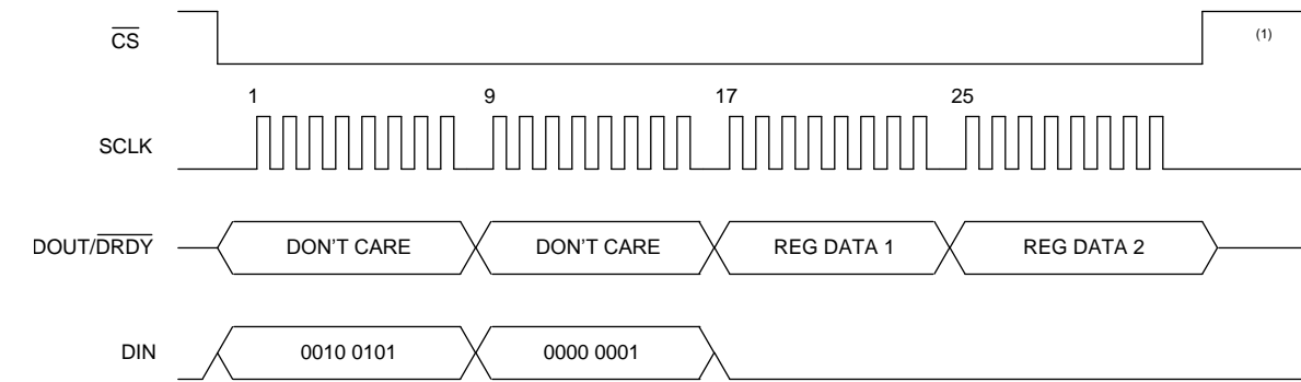
图 88. Read Register Sequence
