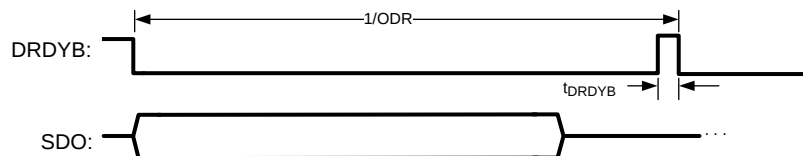
Figure 48. DRDYB Behavior
