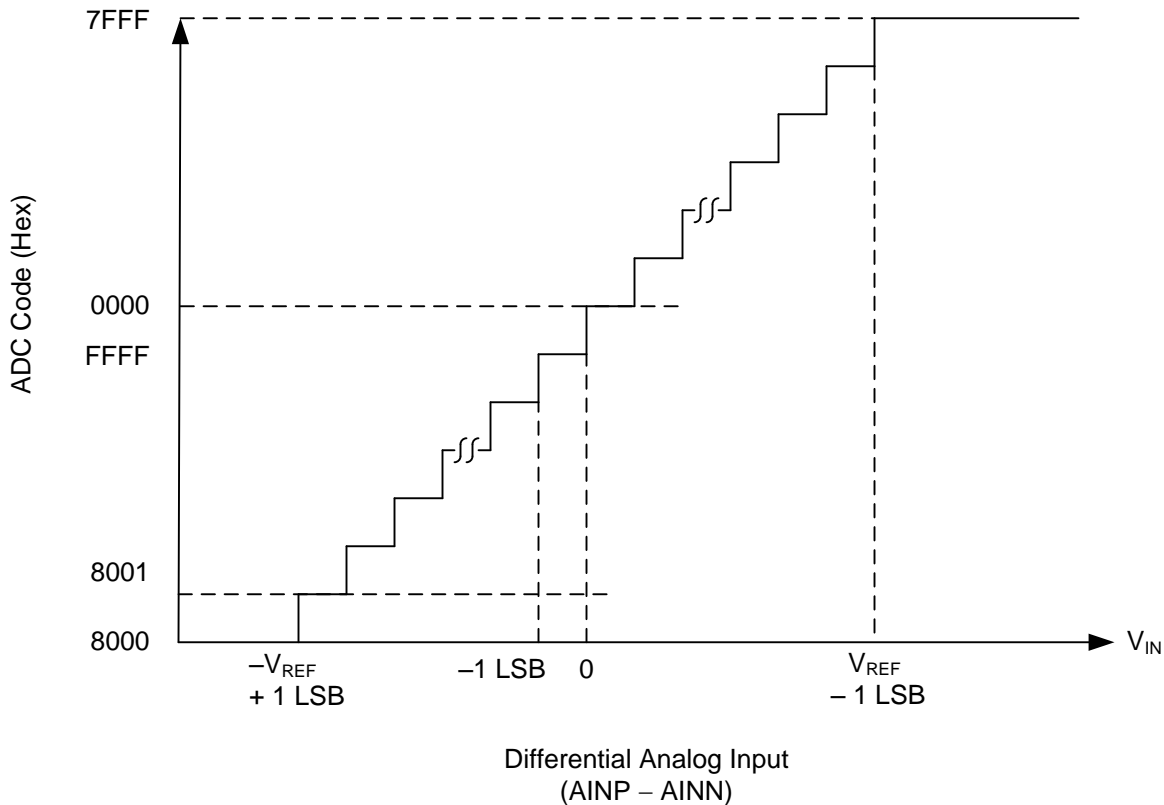
Figure 49. Transfer Characteristics
