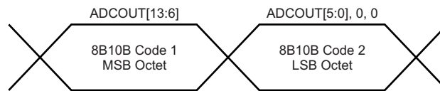
Figure 1. ADC Output Mapping to Two 8B10B Codes
