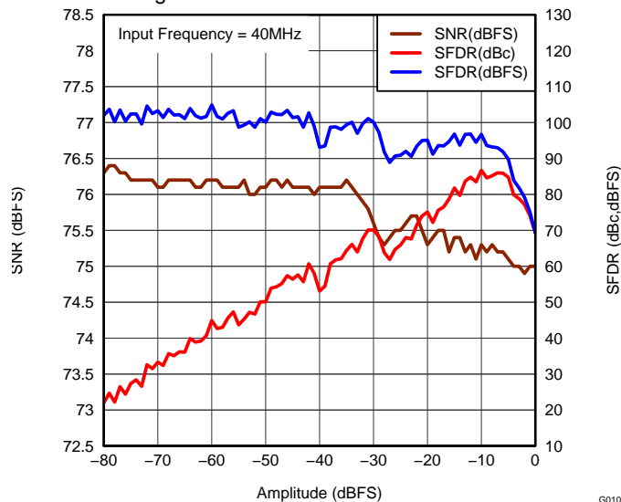
Figure 17. PERFORMANCE ACROSS INPUT AMPLITUDE
