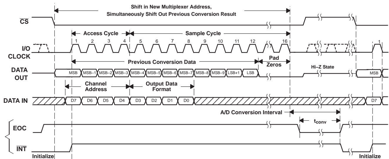
Figure 49. Timing for 8-Clock Transfer Not Using \overline{\text{CS}} With DATA OUT Set for MSB First
