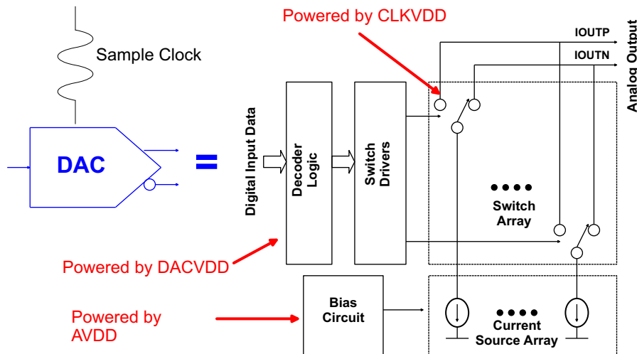
With the DAC34SH84 being a mixed signal device, the device contains circuits that bridges the digital section and the analog section. The DACVDD powers these sections. System designer can design this rail in secondary priority. Powering the rail with LDO is recommended. Unless system designer pays special care to supply filtering and power supply routing/placement, powering the rail directly with switching power supplies is not recommended for this rail.
