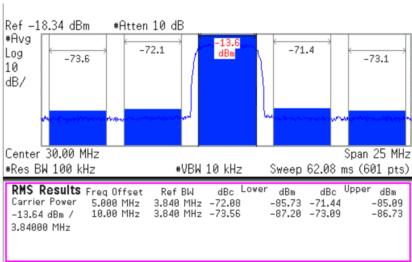
图 9-2. ACPR Performance
