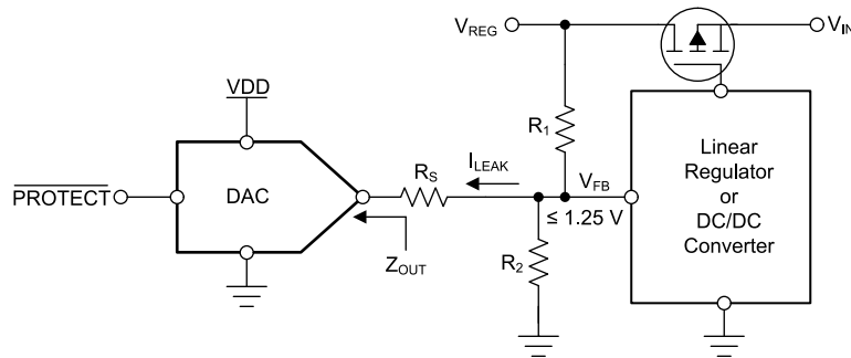
Figure 7-3. High-Impedance (Hi-Z) Output and PROTECT Input
