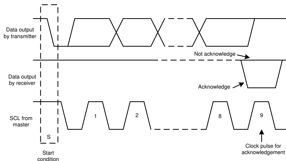
Figure 7-7. Acknowledge and Not Acknowledge on the I 2 C Bus
