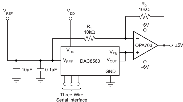
Figure 70. Bipolar Output Range Using External Reference at 5 V
