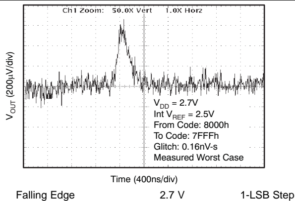
Figure 58. Glitch Energy
