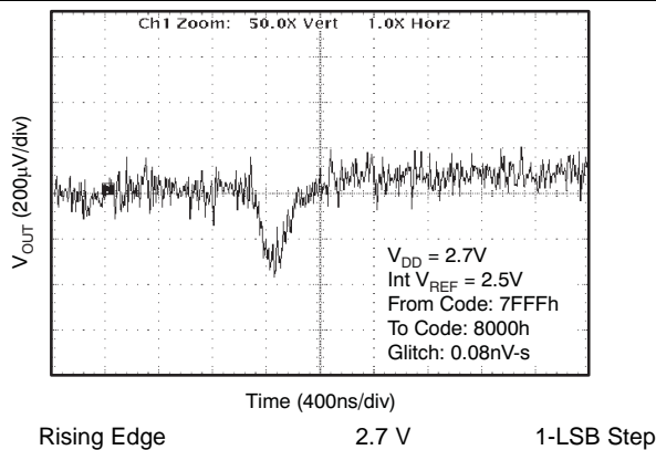
Figure 57. Glitch Energy
