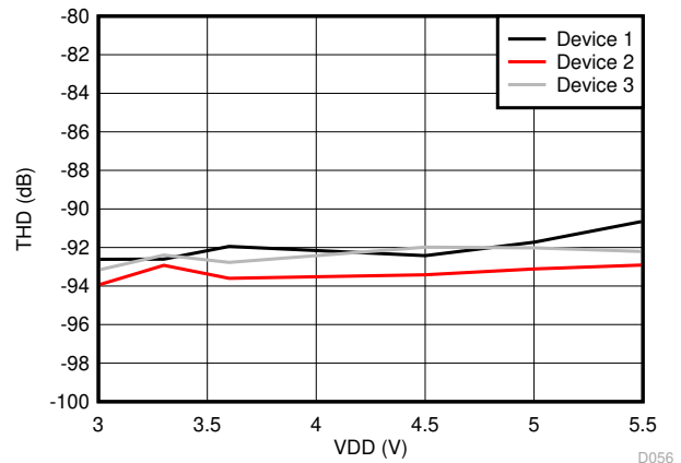
Figure 6-27. Total Harmonic Distortion vs Supply Voltage
