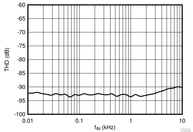
Figure 6-25. Total Harmonic Distortion vs Input Signal Frequency
