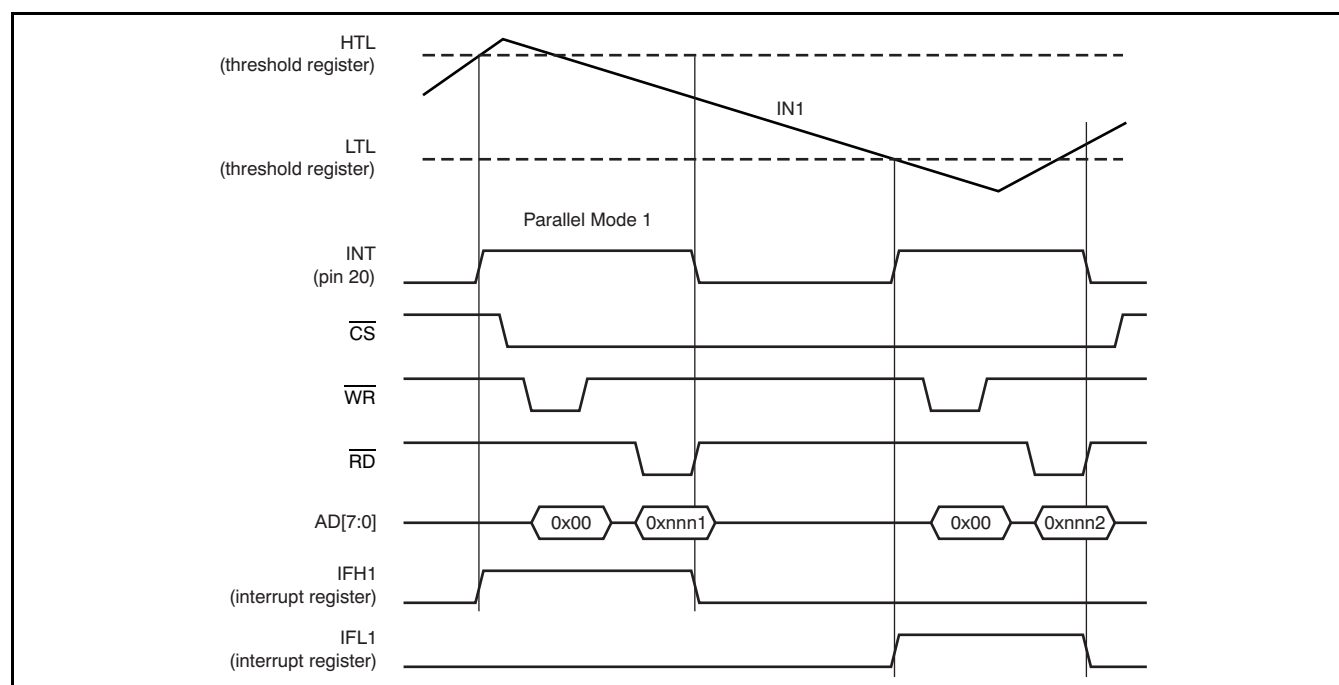
Figure 22. Interrupt Behavior
