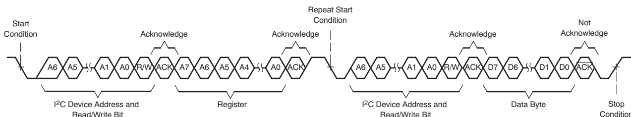
图 85. I 2 C Single-Byte Read Transfer
