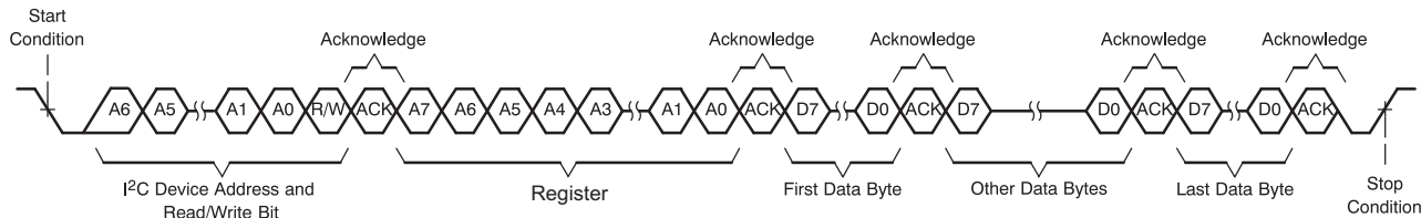
图 84. I 2 C Multiple-Byte Write Transfer
