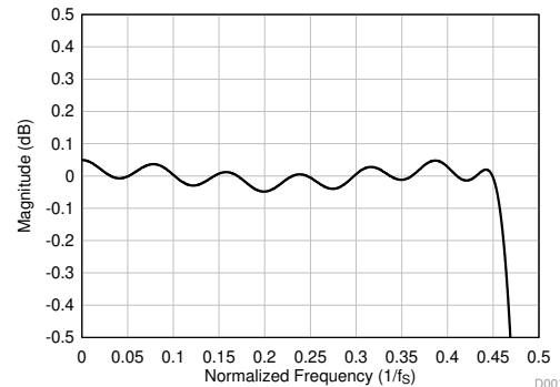
图 46. Linear Phase Decimation Filter Pass-Band Ripple
