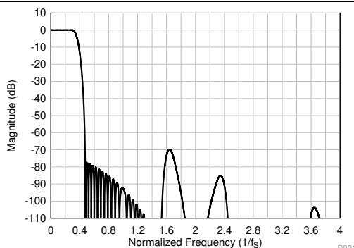
图 47. Linear Phase Decimation Filter Magnitude Response
