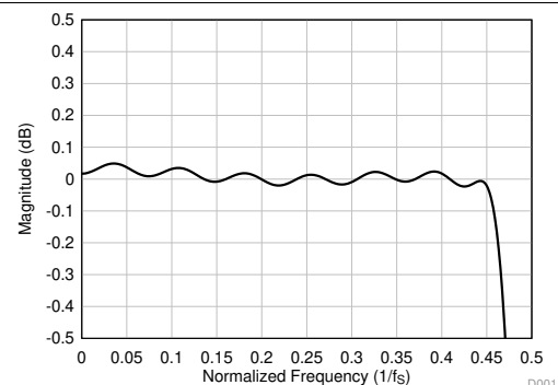
图 36. Linear Phase Decimation Filter Pass-Band Ripple
