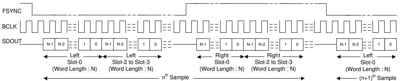
图 21. I²S Mode Standard Protocol Timing (TX_OFFSET = 0)
