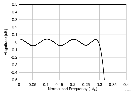
图 48. Linear Phase Decimation Filter Pass-Band Ripple
