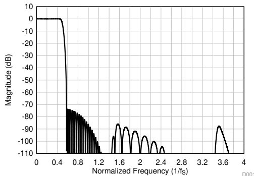
图 45. Linear Phase Decimation Filter Magnitude Response
