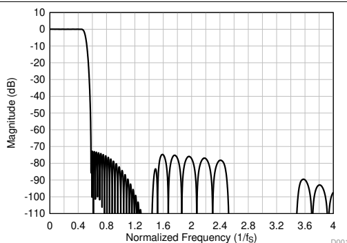
图 35. Linear Phase Decimation Filter Magnitude Response
