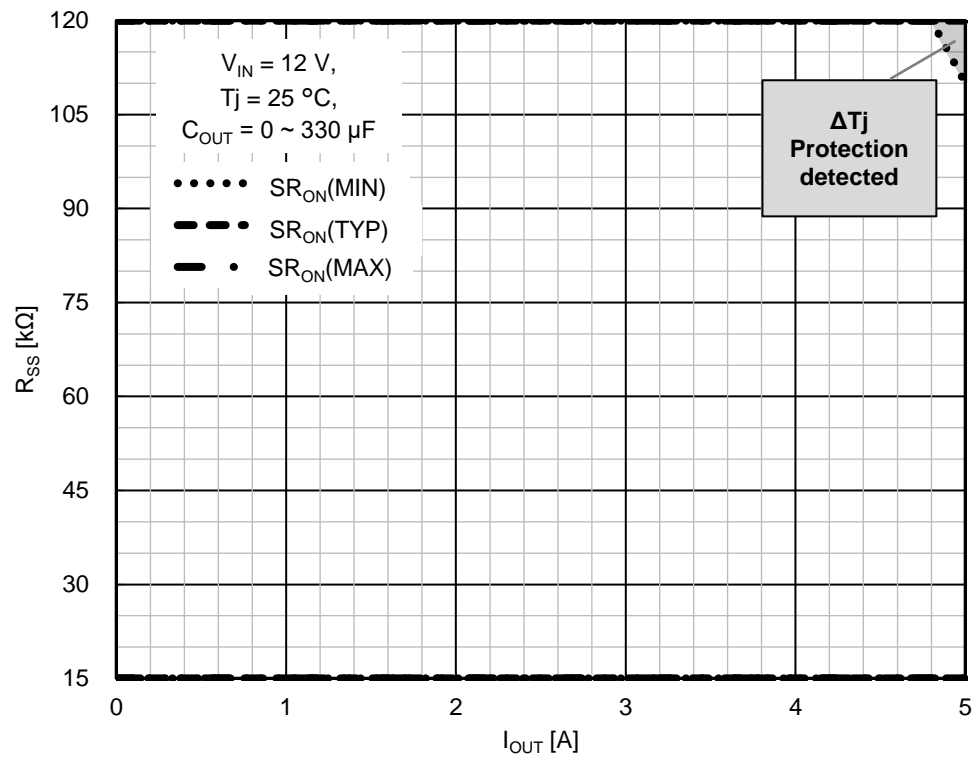
Figure 50. \Delta T_j protection function detection region at startup ( V_{IN} = 12\text{ V}, C_{OUT} = 0 to 470\text{ }\mu\text{F} )
