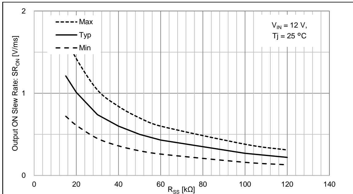
Figure 46. Output ON Slew Rate vs R_{SS} ( V_{IN} = 12\text{ V} , T_j = 25^\circ\text{C} )
