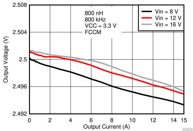
Figure 30. Output Voltage vs Output Current, VCC = 3.3V External Bias
