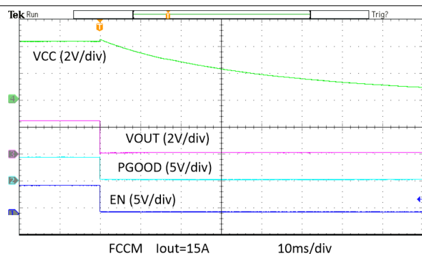
Figure 35. Enable Power Down Full Load
