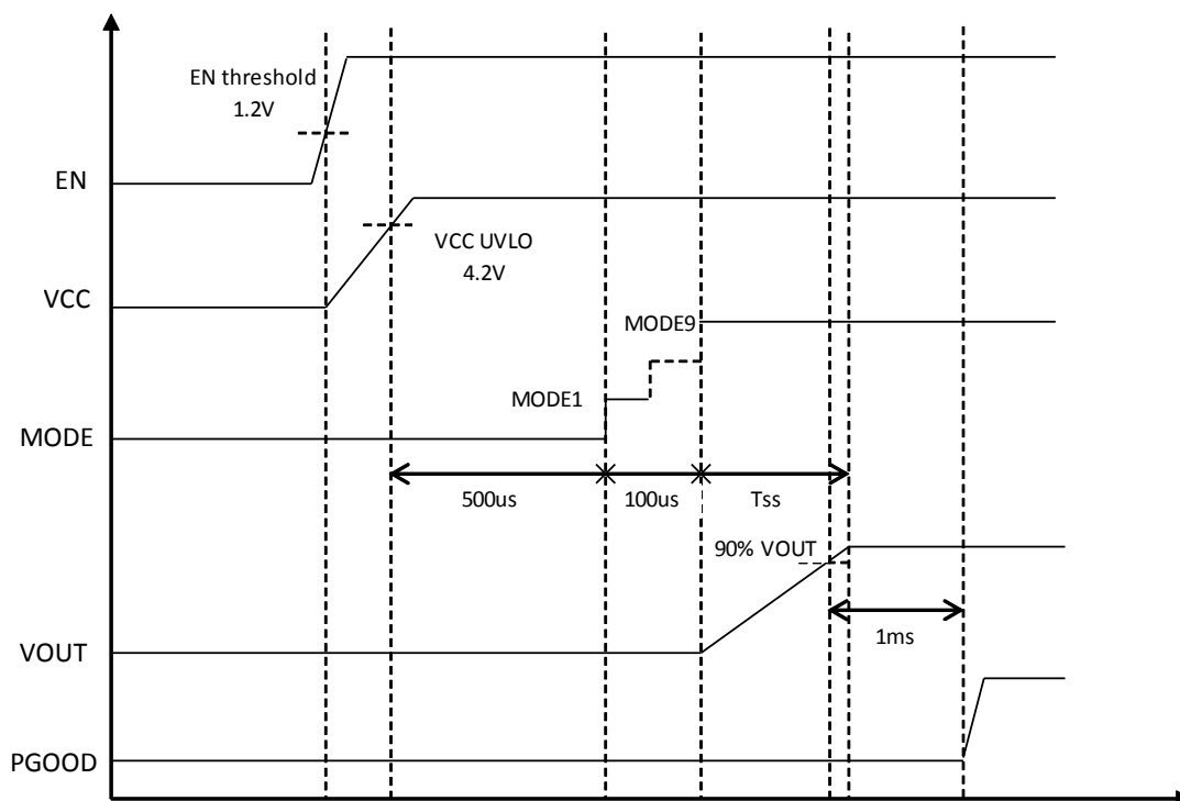
图 29. Power-Up Sequence
