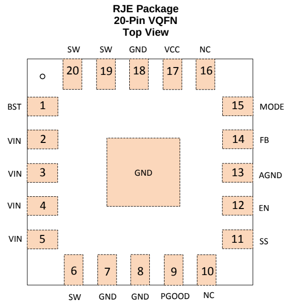
Pin Functions
