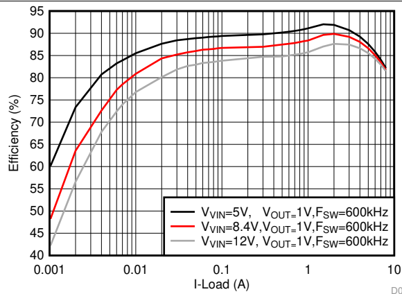
图 31. Efficiency Curve
