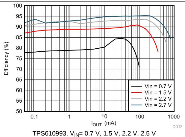
图 6. TPS610993 Load Efficiency with Different Inputs
