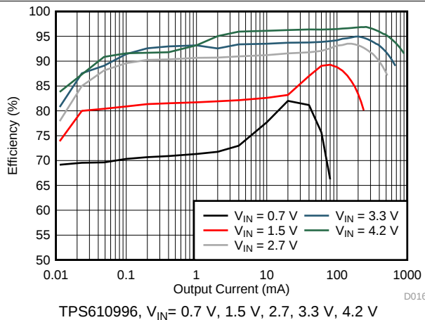
图 3. TPS610996 Load Efficiency with Different Inputs
