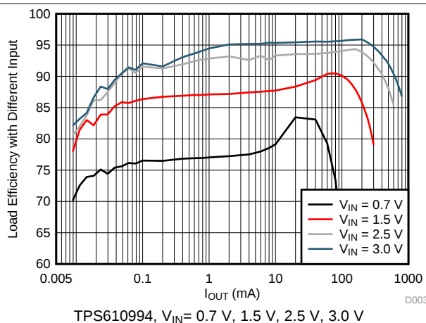
图 5. TPS610994 Load Efficiency with Different Inputs
