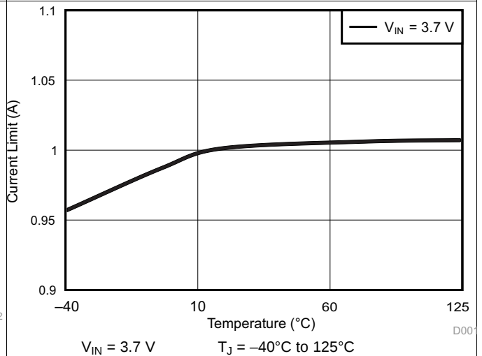
图 16. Current Limit vs Temperature
