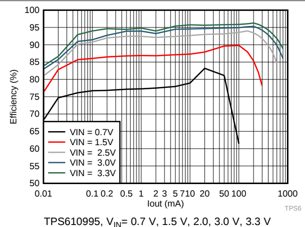
图 4. TPS610995 Load Efficiency with Different Inputs
