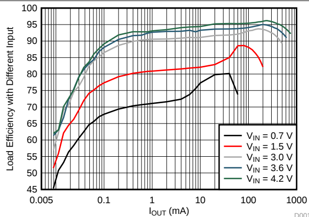
图 1. TPS61099 Load Efficiency with Different Inputs
