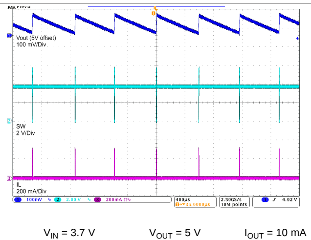
图 22. Switching Waveform at Light Load
