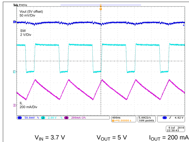
图 21. Switching Waveform at Heavy Load
