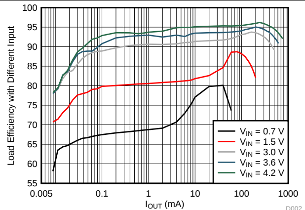
图 2. TPS610997 Load Efficiency with Different Inputs
