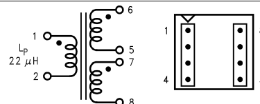
Figure 32. T2 - Top View Coilcraft Q4337-B
