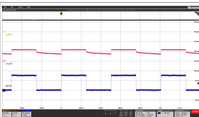
Figure 7-10. LDO Output Load Regulation
