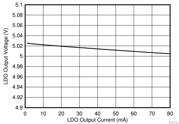
Figure 7-10. LDO Output Load Regulation
