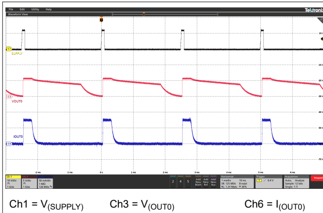
Figure 7-13. Supply Dimming In Fail-Safe Mode
