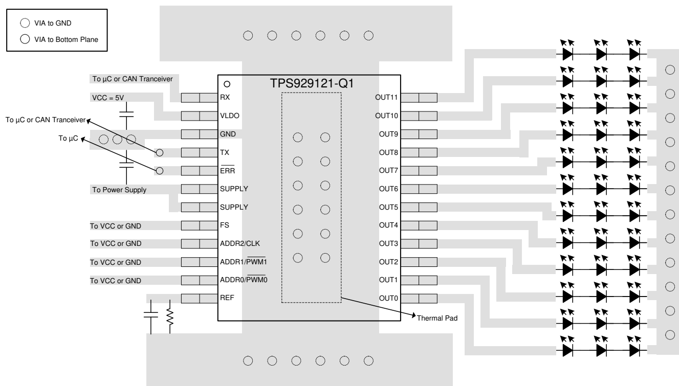
Figure 11-1. TPS929121-Q1 Layout
