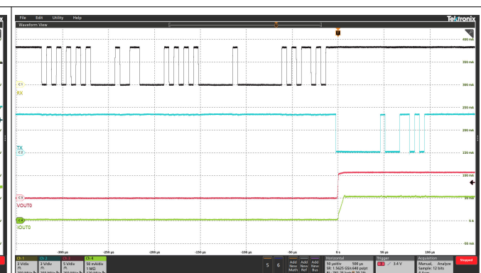
CH1 = RX CH2 = TX CH3 = V_{(\text{OUT0})} CH4 = I_{(\text{OUT0})}
