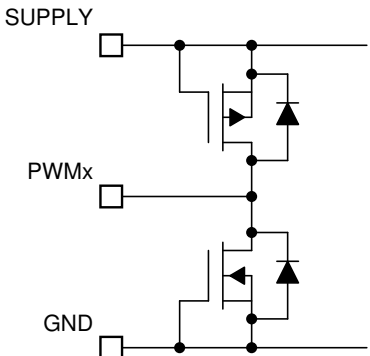
图 7-15. PWM1, PWM2 and PWM3 Pins
