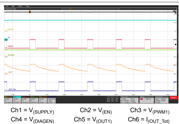
图 8-6. PWM Dimming 20% Dutycycle at 600 Hz
