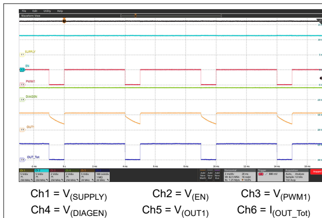
图 8-5. PWM Dimming 80% Dutycycle at 200 Hz
