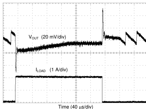
Figure 8-19. Transient from PWM-to-PFM Mode
