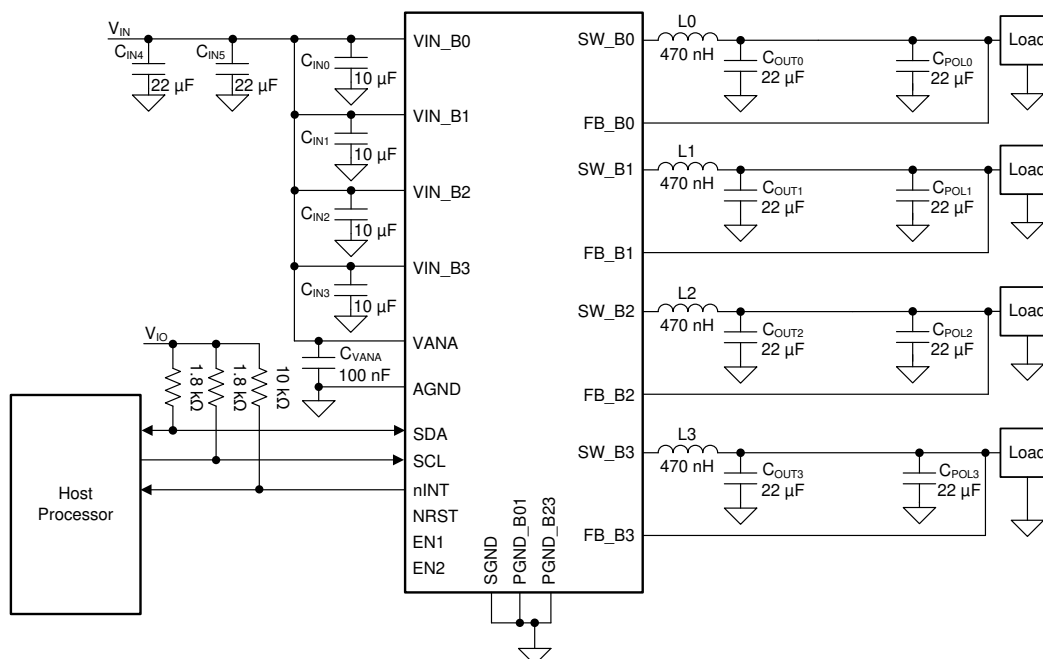
Figure 8-1. LP8758-EA Typical Application Circuit
