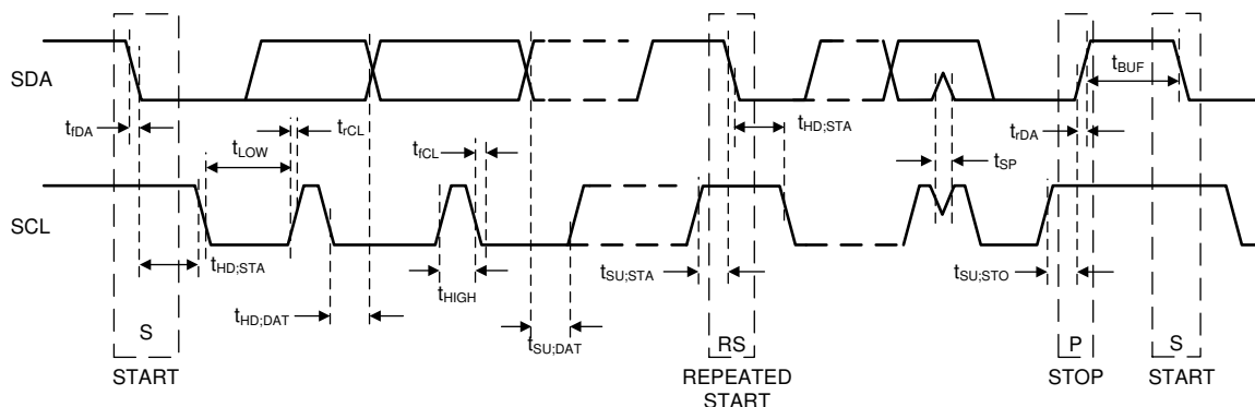
Figure 7-10. I²C-Compatible Timing
