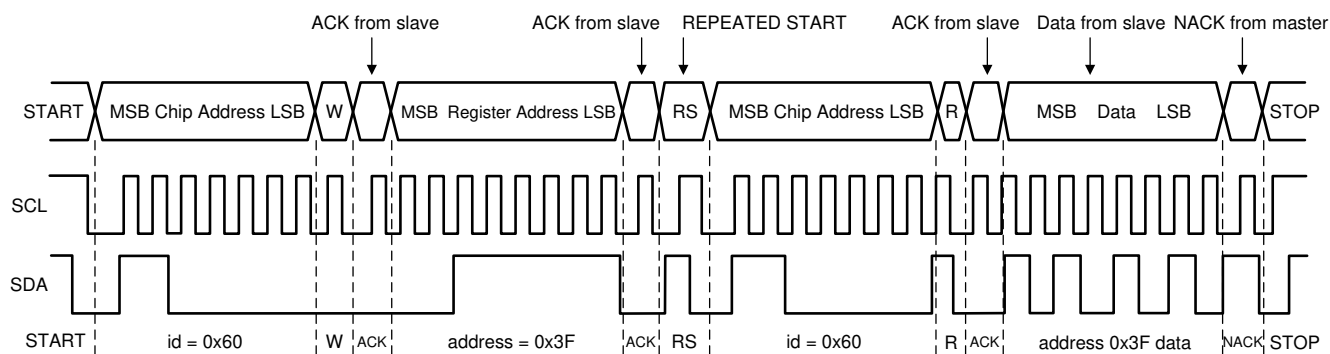
Figure 7-12. Read Cycle ( r = read; SDA = 1), id = Device Address = 60Hex for LP8758-EA
