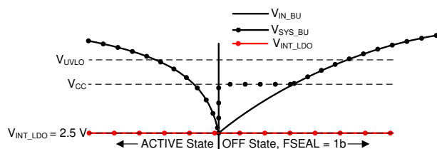
Figure 8-18. Switching Behavior of the Battery-Backup-Supply Power-Path; Power-Path Hysteresis
