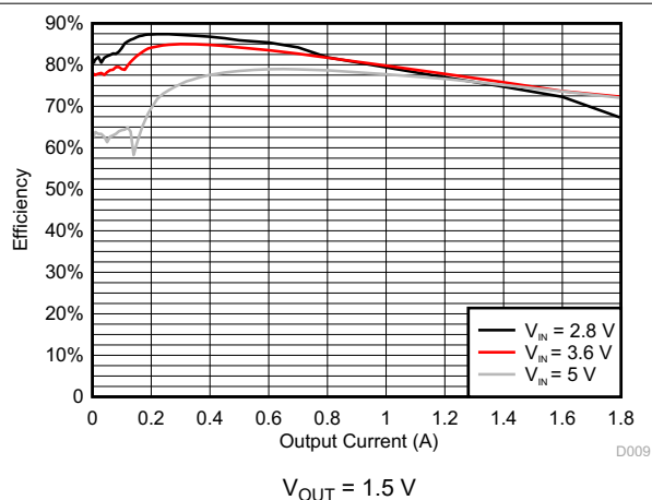
Figure 9-6. DCDC3 Efficiency
