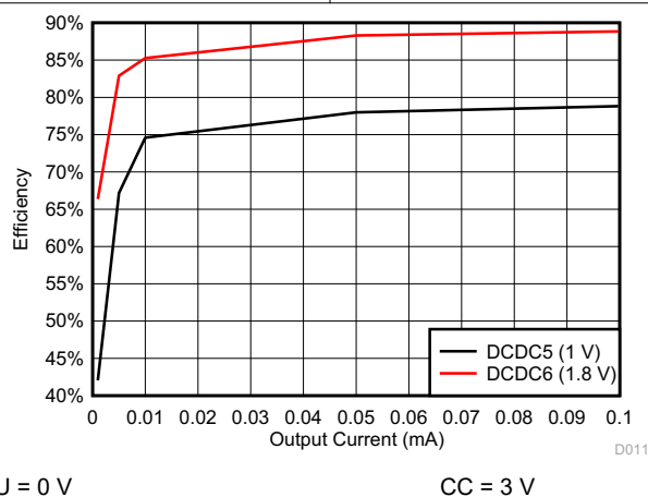
Figure 9-8. DCDC5/DCDC6 Efficiency
