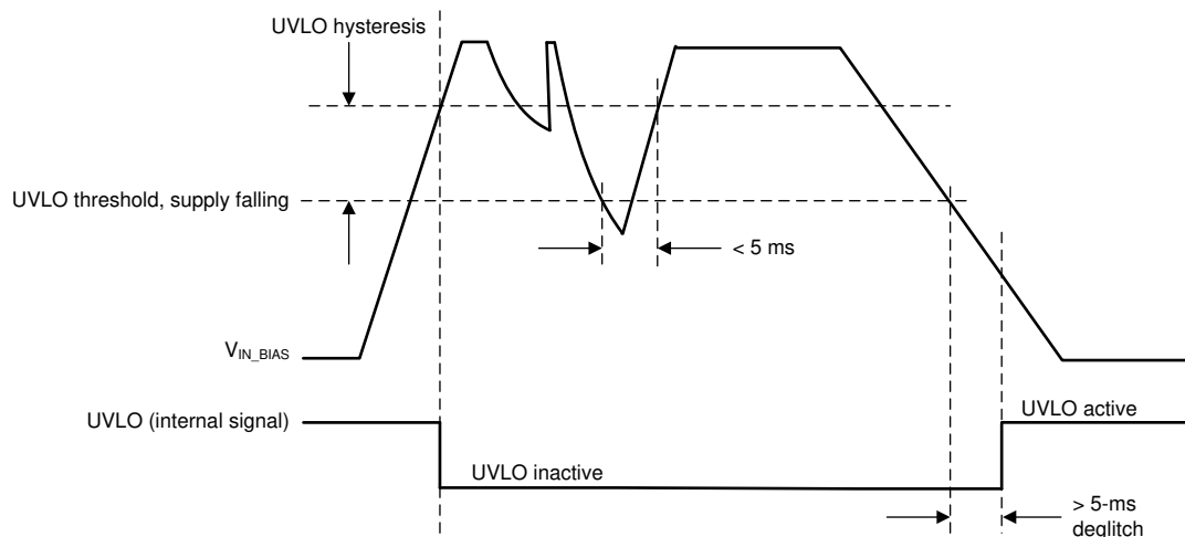
Figure 8-16. Definition of UVLO and Hysteresis, IN\_BIAS Slew Rate < 30\text{ V/s}
