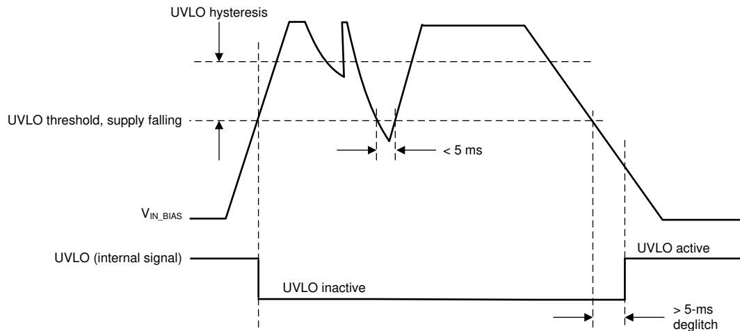
Figure 8-15. Definition of UVLO and Hysteresis, IN\_BIAS Slew Rate > 30\text{ V/s}
