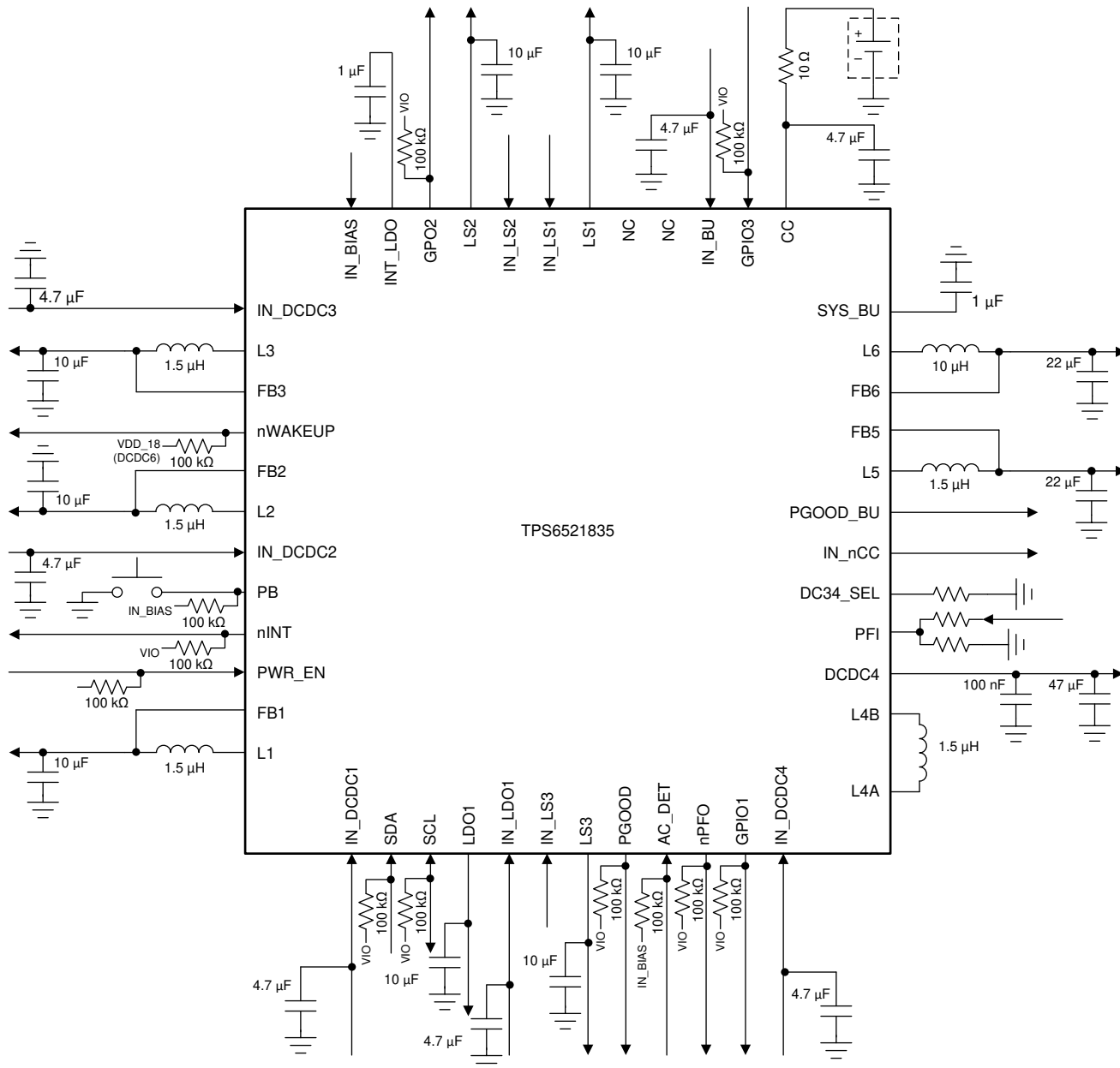
Figure 4-1. Simplified Schematic
