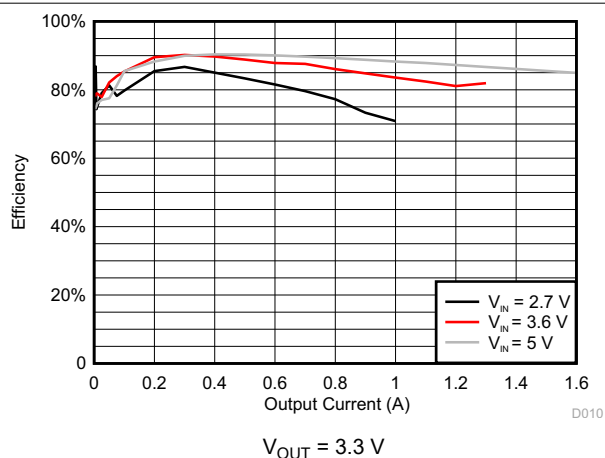
Figure 9-7. DCDC4 Efficiency
