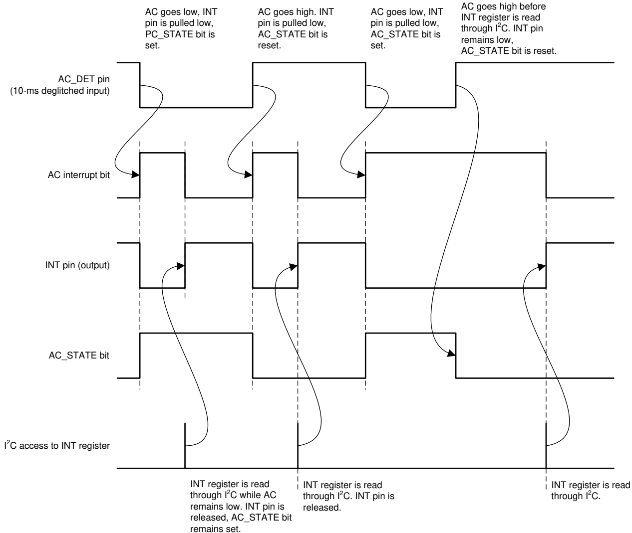
Figure 8-30. AC_STATE Pin
