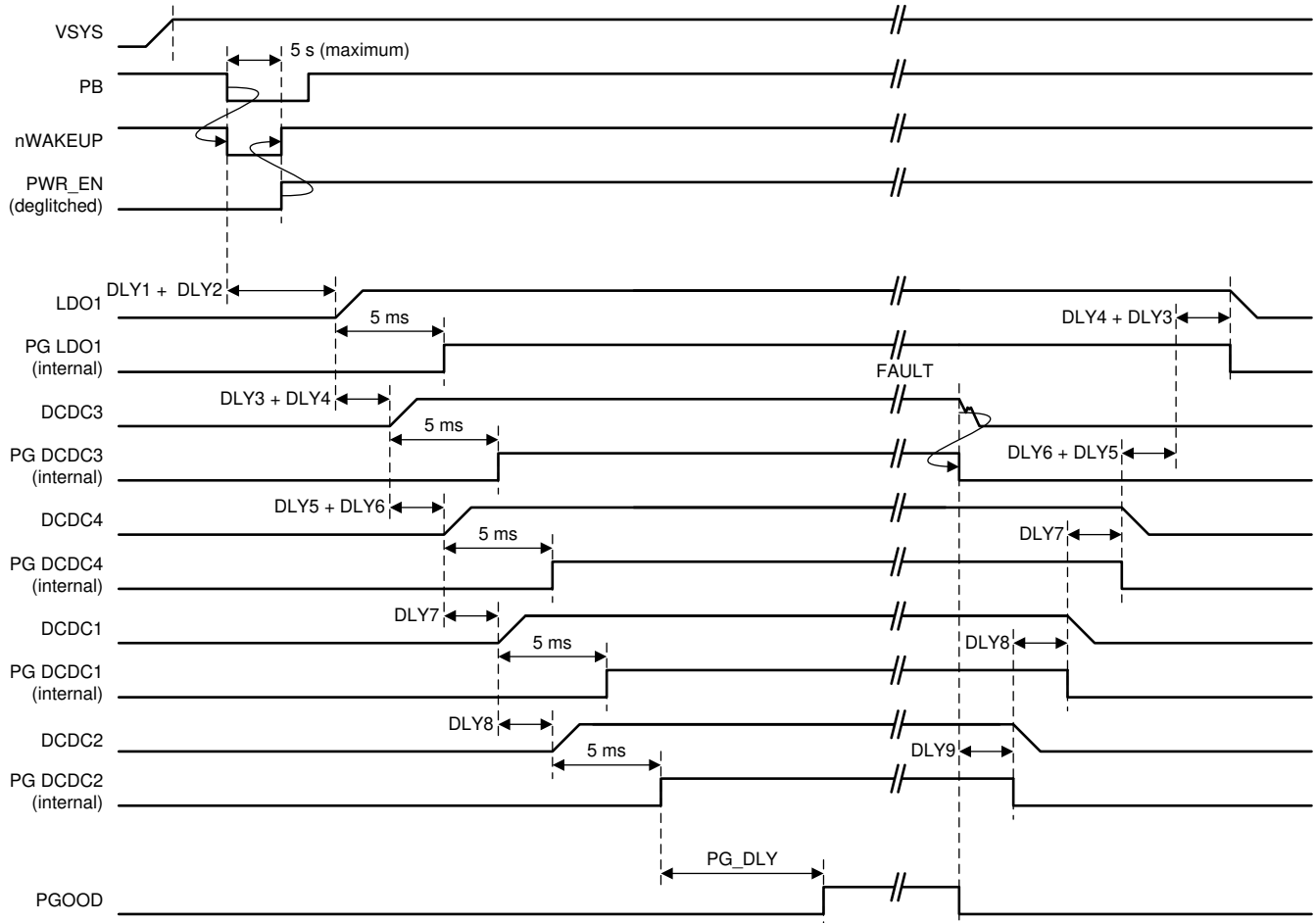
Figure 8-8. Typical Power-Up Sequence of the Main Output Rails
