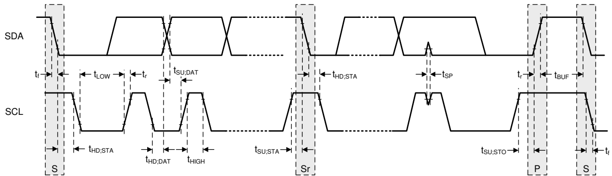
Figure 8-34. I²C Protocol and Transmission Timing I²C Data Transmission Timing
