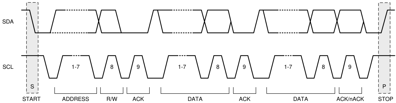
Figure 8-33. I²C Protocol and Transmission Timing I²C Start Stop and Acknowledge Protocol
