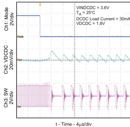
Figure 14. PWM to PFM Transition (DC-DC)
