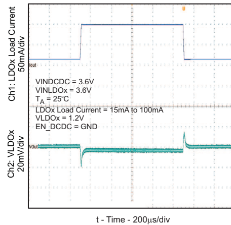
Figure 12. Load Transient Response (LDOx)
