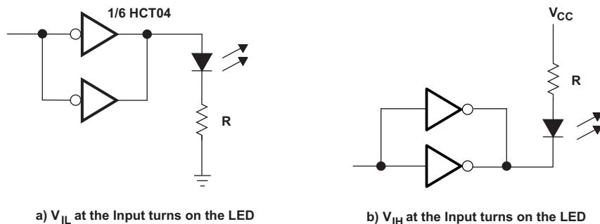
Figure 4. Driving LEDs
