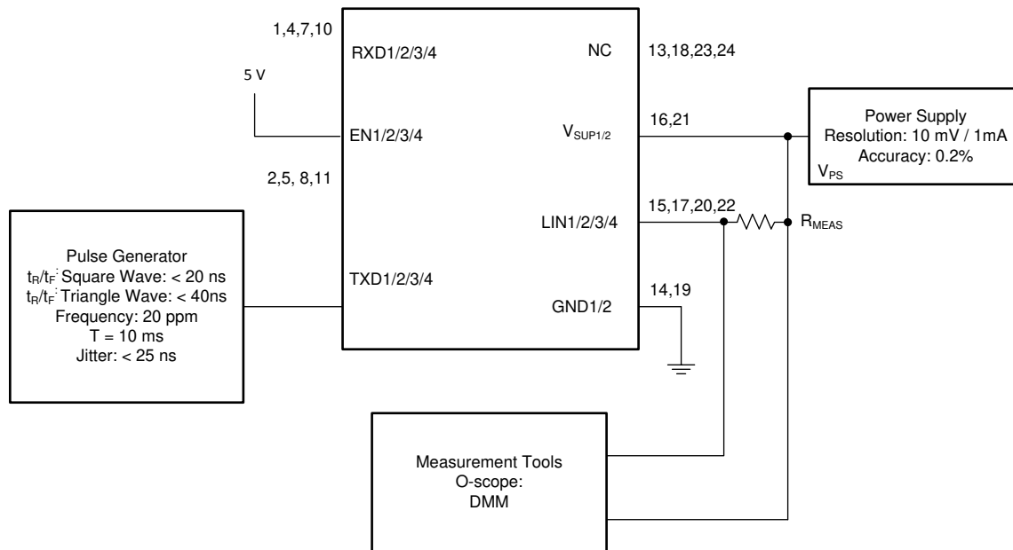
图 13. Test Circuit for I_{BUS\_LIM} at Dominant State (Driver on)
