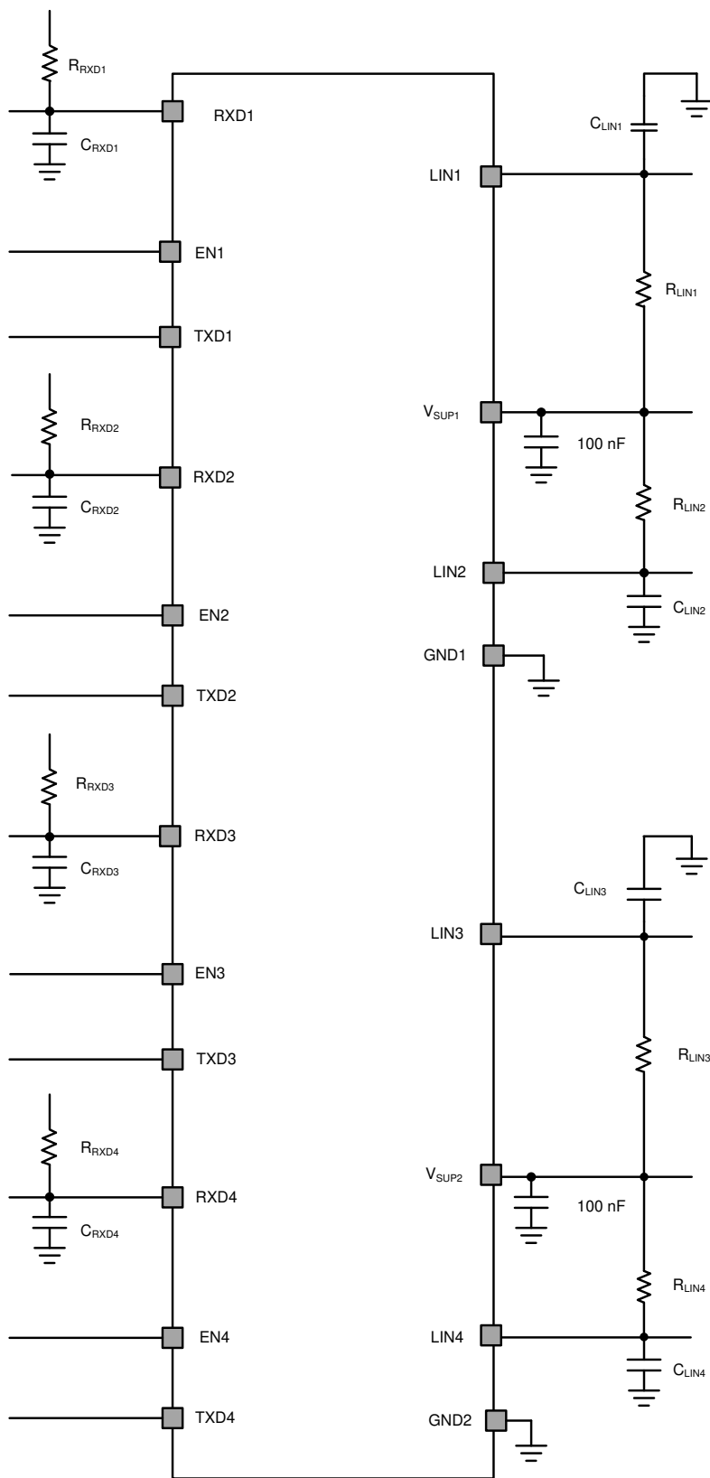
图 25. Test Circuit for AC Characteristics
