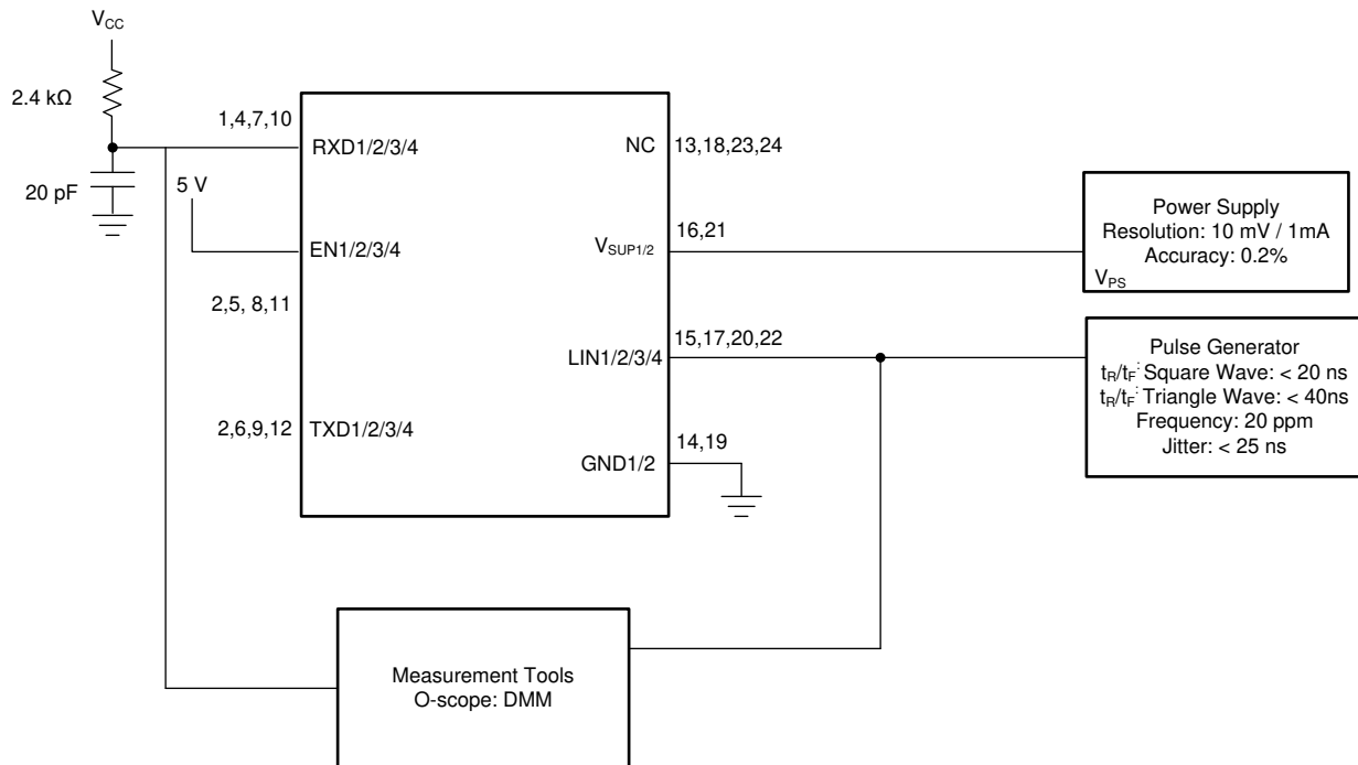
图 20. Propagation Delay Test Circuit
