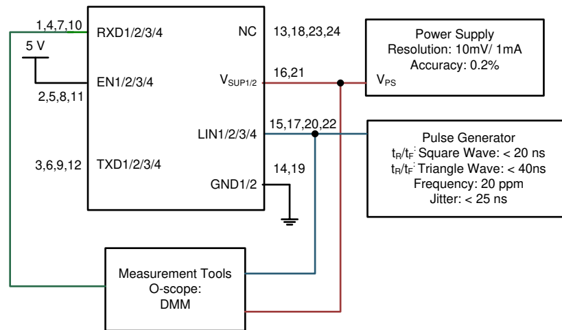
图 8. Test System: Operating Voltage Range with RX and TX Access
