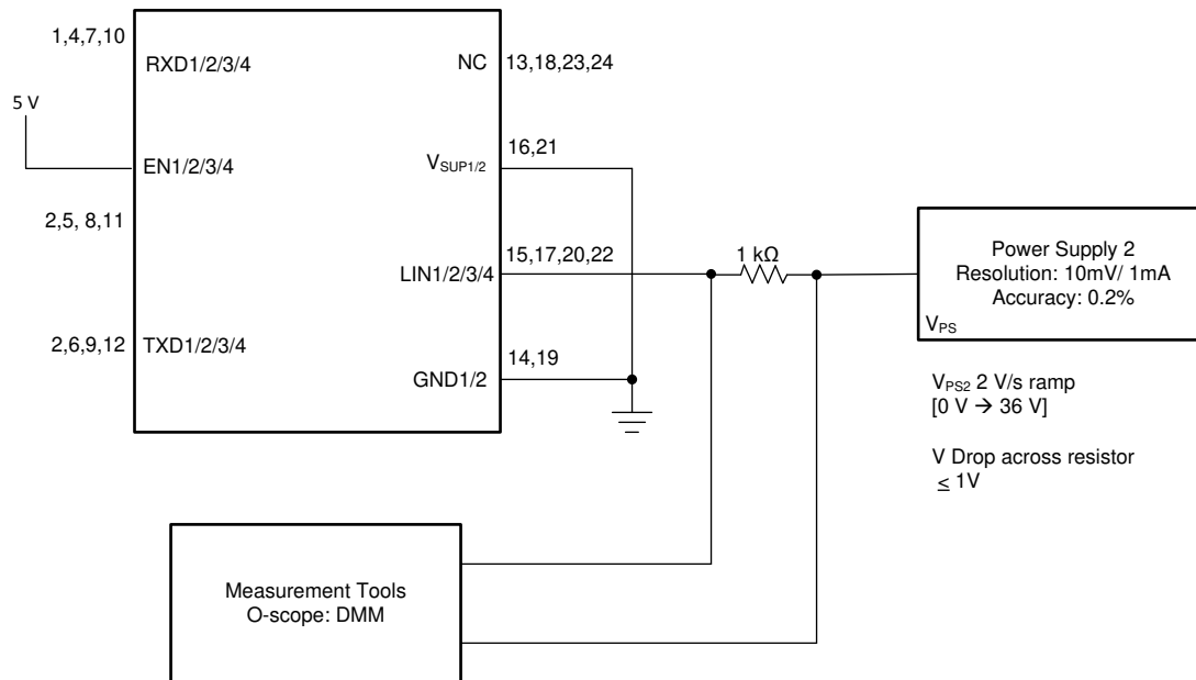
图 17. Test Circuit for I_{BUS\_NO\_BAT} Loss of Battery
