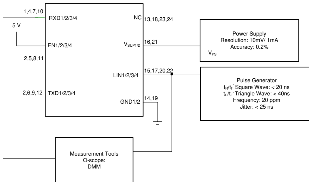
图 11. LIN Receiver Test with RX Access
