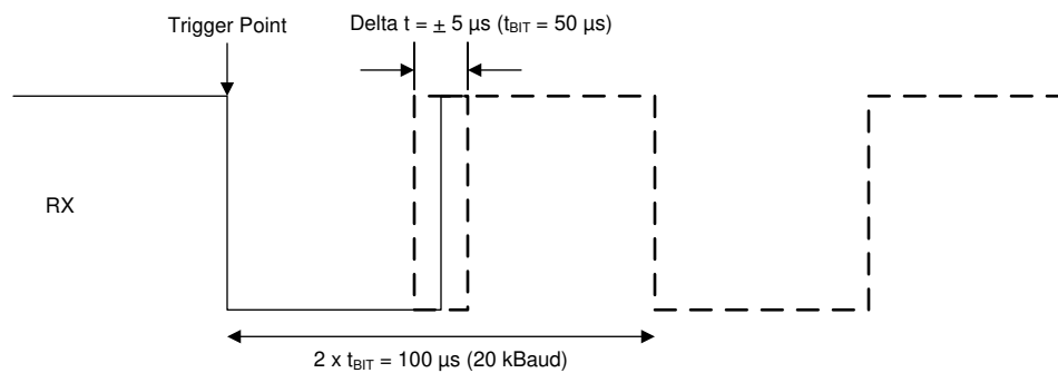
图 9. RX Response: Operating Voltage Range
