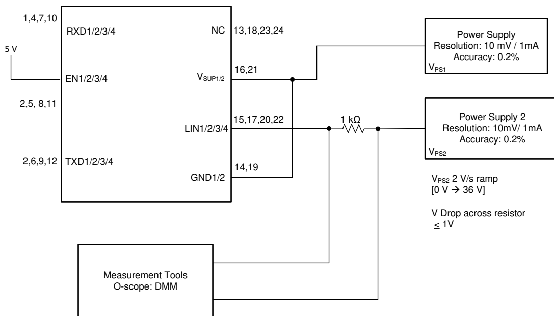
图 16. Test Circuit for I_{BUS\_NO\_GND} Loss of GND
