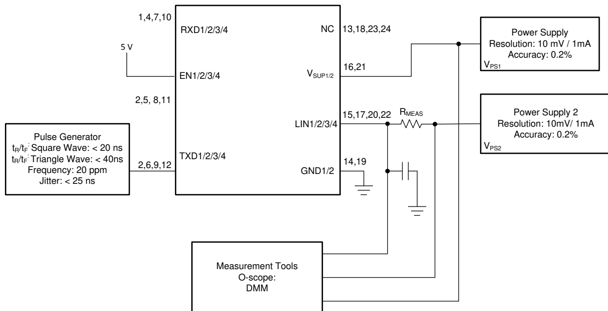
图 18. Test Circuit Slope Control and Duty Cycle
