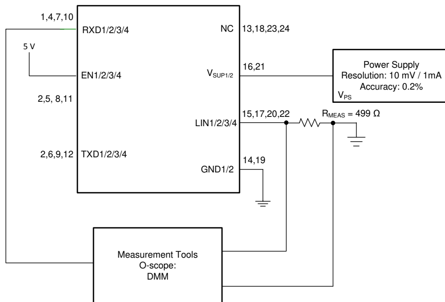
图 14. Test Circuit for I_{BUS\_PAS\_dom} ; TXD = Recessive State V_{BUS} = 0 V
