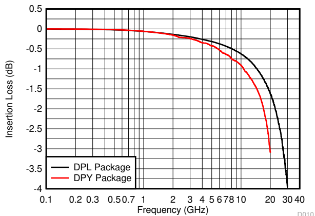
Figure 8-4. Insertion Loss
