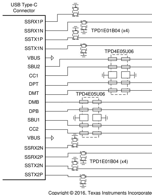
Figure 8-1. USB Type-C for Thunderbolt 3 ESD Schematic
