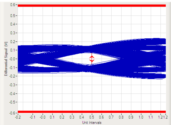
Figure 8-2. USB 3.1 Gen 2 10-Gbps Eye Diagram (Bare Board)
