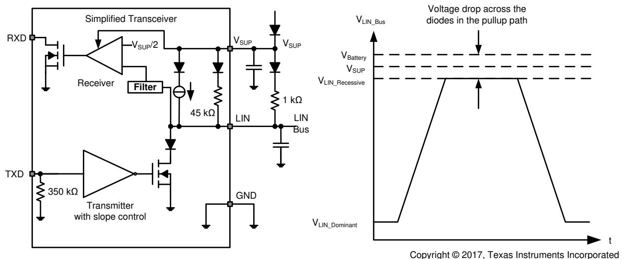
图 8-1. Leader Node Configuration with Voltage Levels
