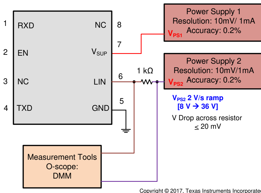
图 7-8. Test Circuit for I_{BUS\_PAS\_rec} Param 14
