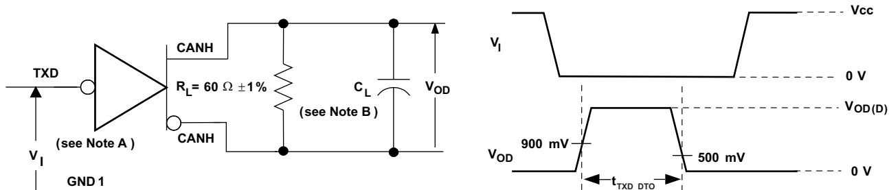
图 16. Dominant Time-out Test Circuit and Voltage Waveforms
