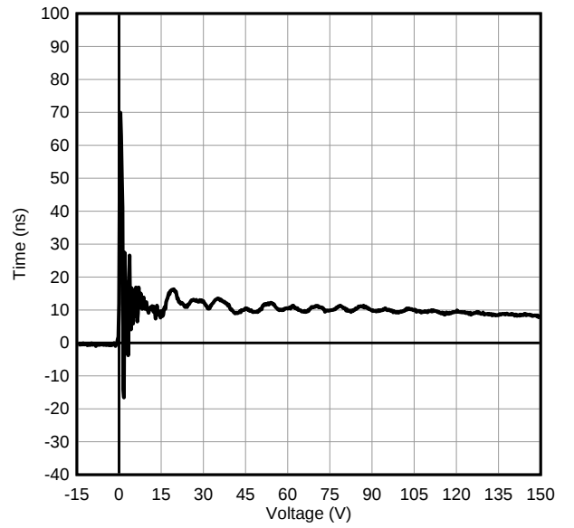
Figure 5. IEC 61000-4-2 Voltage Clamp Waveform 8-kV Contact
