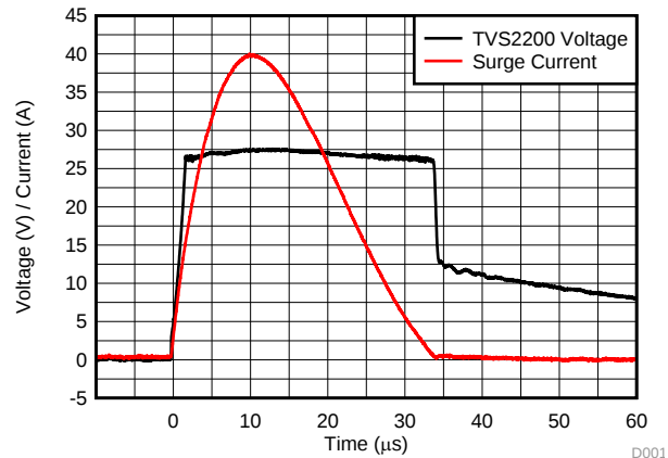
图 11. TVS2200 Surge Response at 40 A
