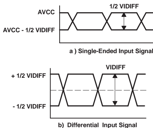
Figure 15. TMDS Inputs
