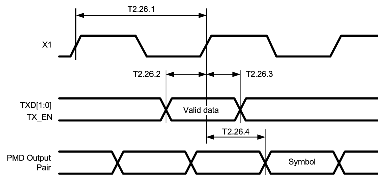
Figure 4-24. RMII Transmit Timing
