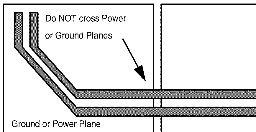
图 22. Differential Signal Pair and Plane Crossing
