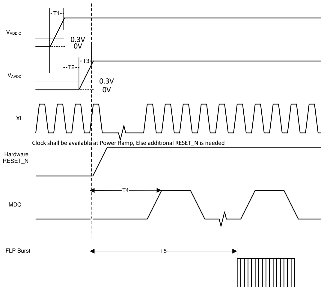
图 1. Power-Up Timing
