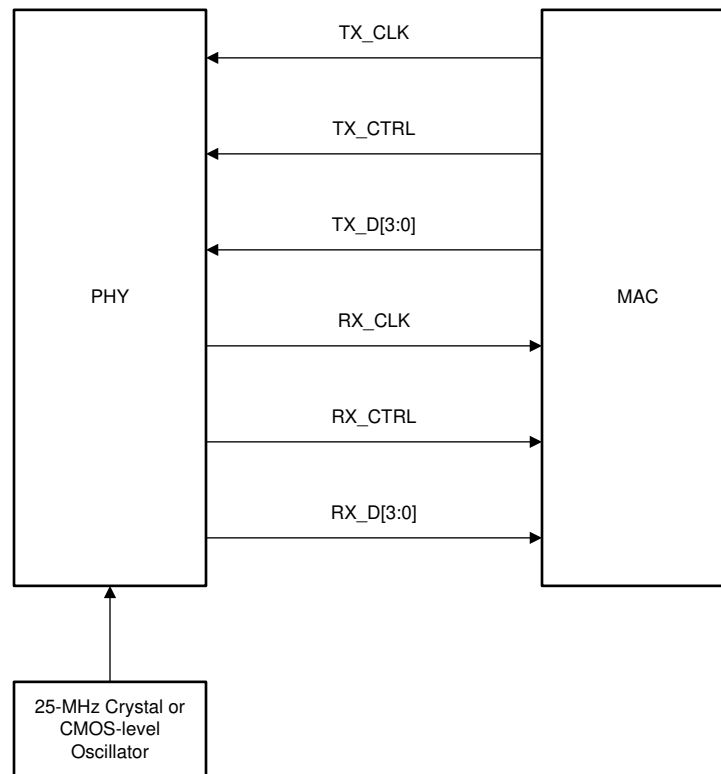
Figure 7-13. RGMII Connections
