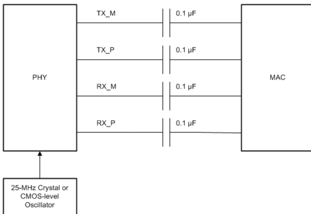
Figure 7-16. SGMII Connections
