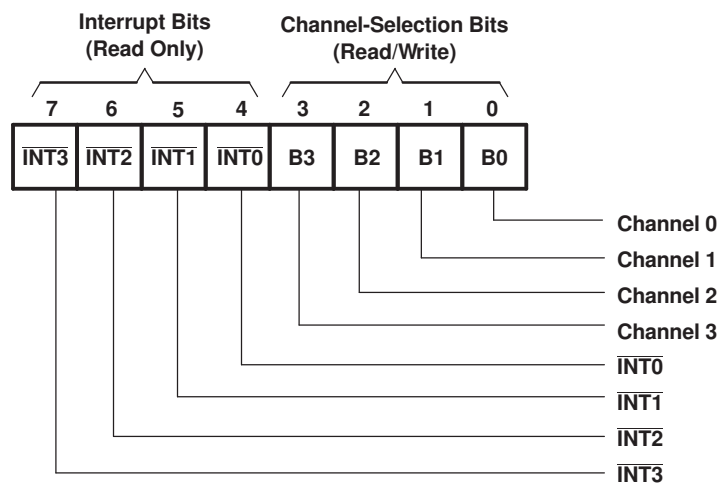
Figure 15. Control Register
