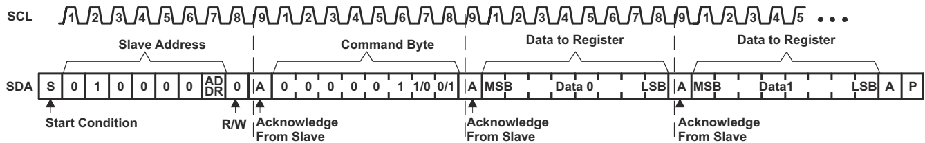
图 8-9. Write to Configuration or Polarity Inversion Registers
