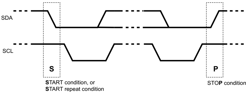
Figure 23. START and STOP Conditions
