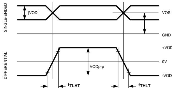
Figure 9. FPD-Link (LVDS) Single-ended and Differential Waveforms
